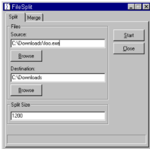
Figure 1. FileSplit window
