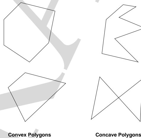
Figure 5.3: Polygons
