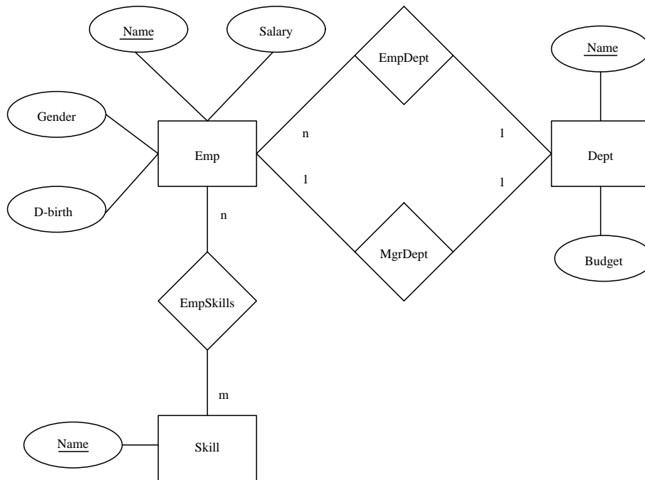
Figure 1: ER Diagram of Database Design
