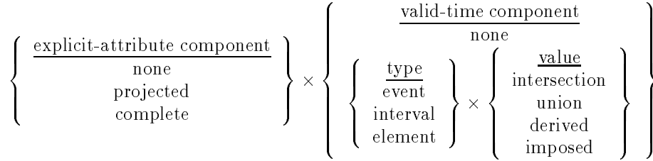
Figure 4: Output-based Taxonomy
