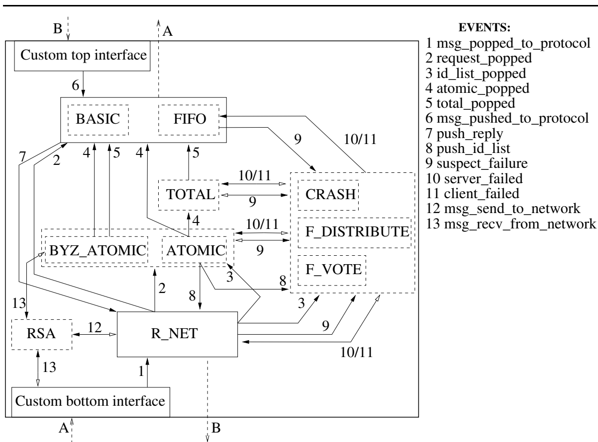
Figure 2: Server micro-protocols
