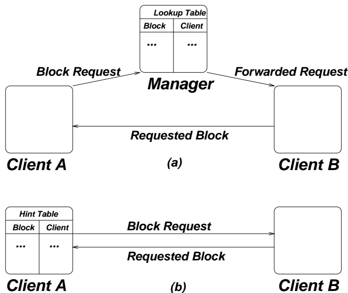
Figure 2.3: Locating Blocks in the Client Caches. This figure shows two possible approaches for locating blocks in the client caches. Part (a) shows the manager-centric approach, where a client contacts a manager on a local cache miss. The manager consults its lookup table and forwards the block request to the client caching the block. This client provides the block to the requesting client. Part (b) shows the hint-based approach, where on a local cache miss, a client consults its hint table and directly contacts the client caching the block. This client provides the block to the requesting client, avoiding the overhead of contacting the manager. Of course, the success of the hint-based approach depends on the accuracy of hints.
