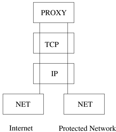
Figure 2: Overview of an application-level firewall. Data from one network pass through the proxy which forwards them to the other network if the desired security guarantees are not violated.
