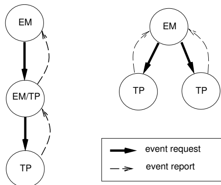
Figure 11.1: Monitoring a monitor; monitoring multiple TPs
