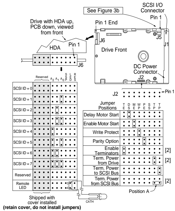
Figure 3a. Drive configurator, Hawk 2LP family N/ND models
