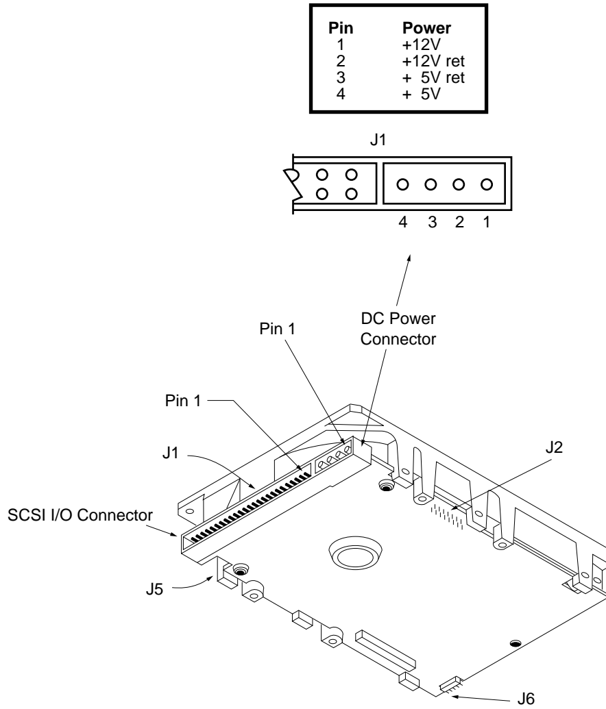
Figure 11.6-1. Physical interface
