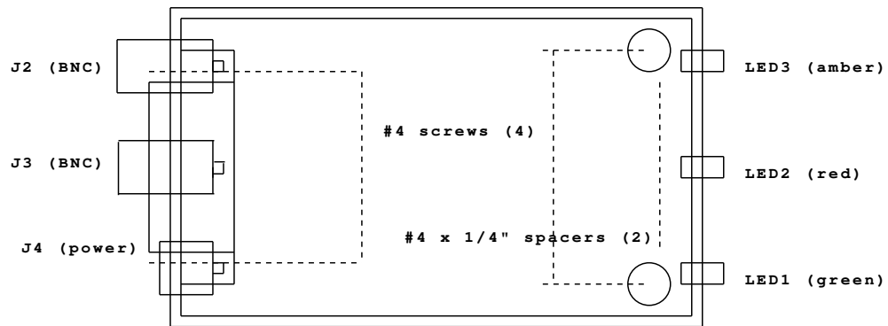
Top View (cover removed)
