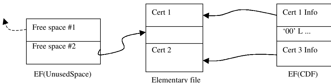
Figure 15 – After removing certificate 2
