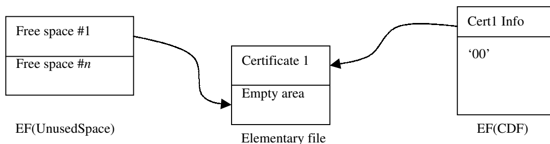
Figure 12 – Before adding a new certificate
