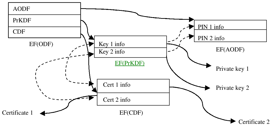
Figure 16 – IC card file relationships in DF(PKCS15). Dashed arrows indicate cross-references.
