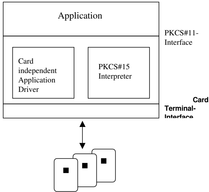
Figure 1 – Embedding of a PKCS #15 interpreter (example)
