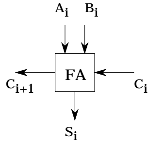
Full-Adder Cell
