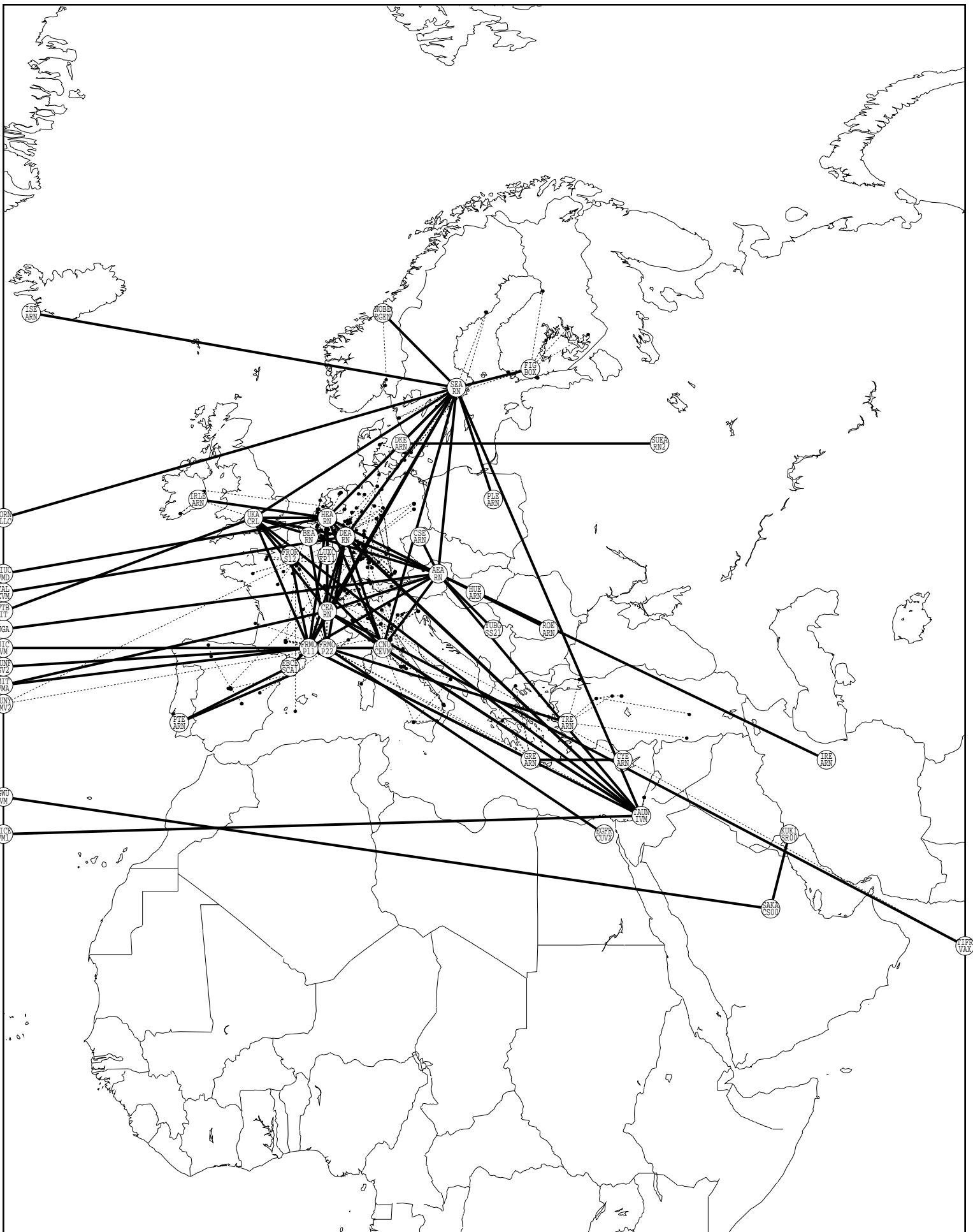
BITNET/EARN connectivity in Europe/MidEast/Africa All published network links shown
