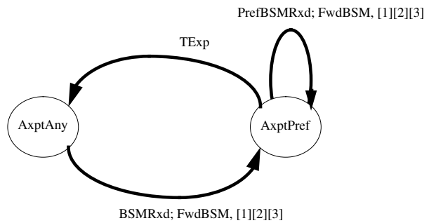
State transition diagram for a router not configured as C-BSR
