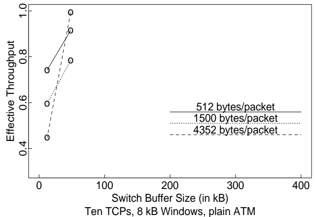
Figure 2: TCP over Plain ATM
