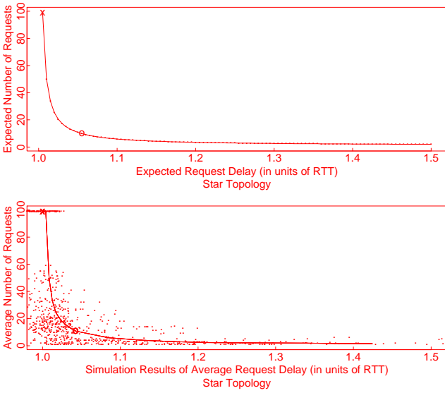
Figure 7: Tradeoff between delay and duplicates in a star topology.
