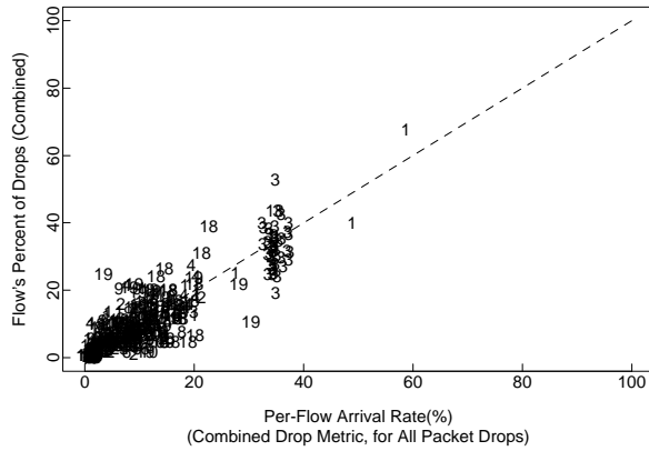
Figure 5: The combined drop metric for all packet drops.
