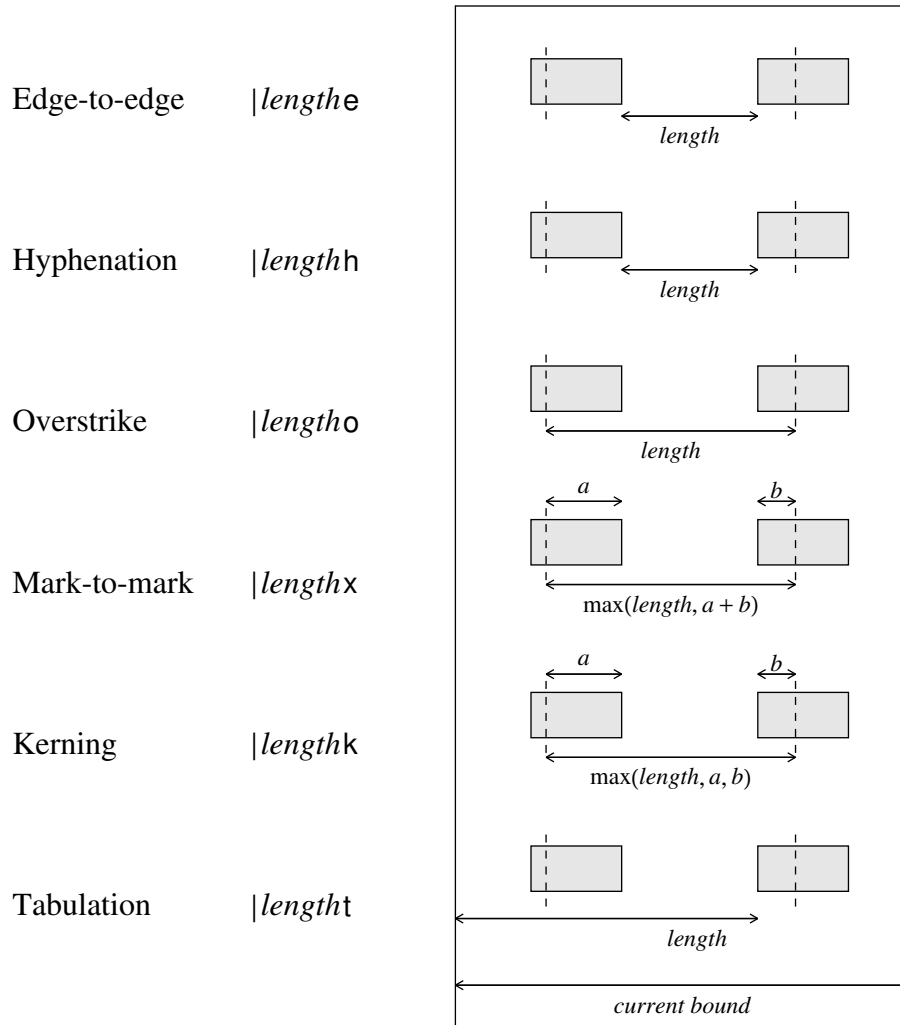
Figure 2. The six gap modes ( length is any length). Hyphenation mode has an extra property not shown here.
