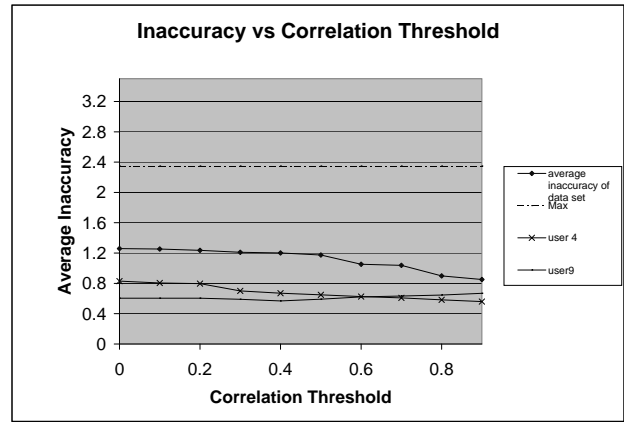
Figure 1: Plot showing the relationship between the average inaccuracy and the correlation threshold for data from the Each-Movie Data. This dataset consists of the ratings of 58 users and one 125 movies. Average inaccuracy is an average of the differences between the rating and the prediction for every pair of users and movies in the data set.
