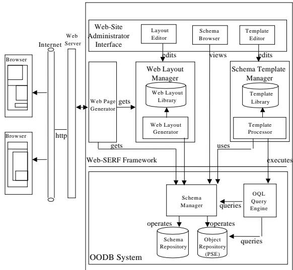
Figure 2: Architecture of the Re-WEB Framework.
