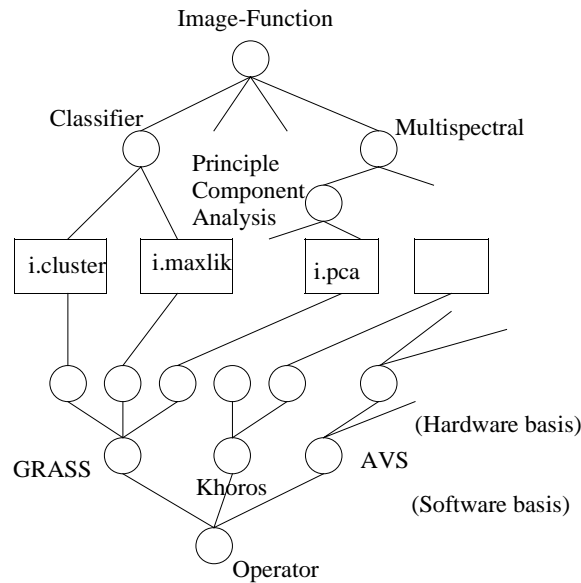
Figure 5: Operator taxonomies
