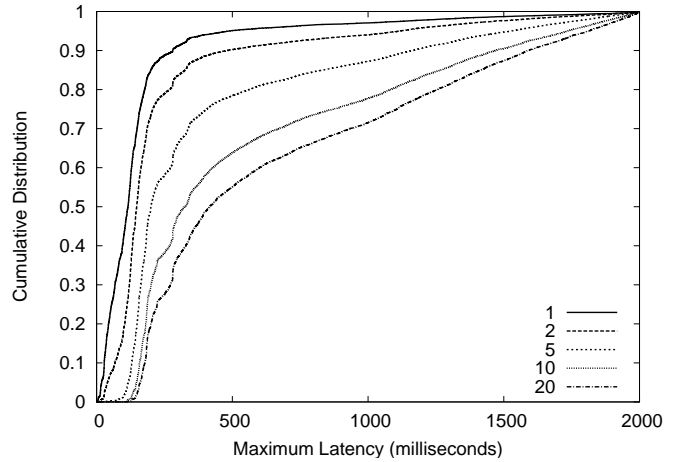
Figure 12: Cumulative Distribution of Maximum Ping for Different Numbers of Clients Playing Together
