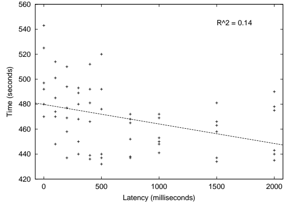
Figure 13: Age of Mythology - Build Time versus Latency.
