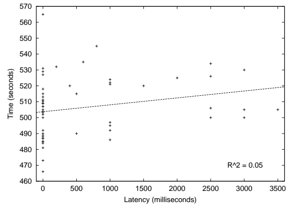
Figure 4: Warcraft III - Build Time versus Latency.
