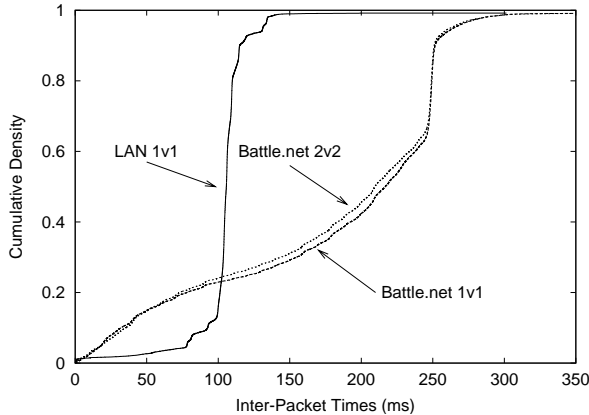
Figure 11: Warcraft III - Inter-packet Distributions.
