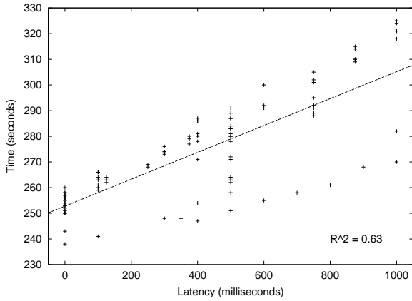
Figure 5: Warcraft III - Explore Time versus Latency.
