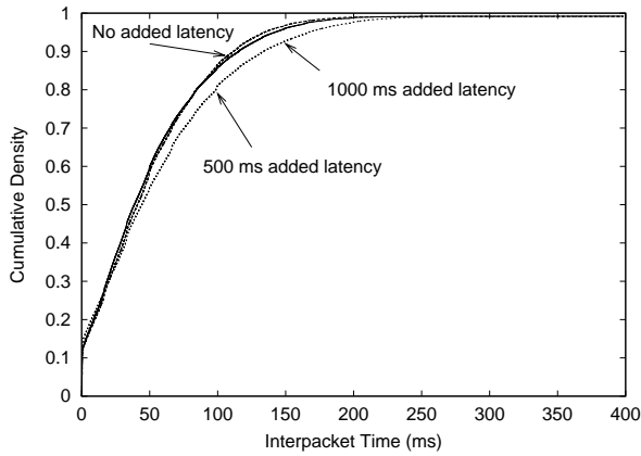
Figure 23: Age of Mythology - Inter-packet Distributions.
