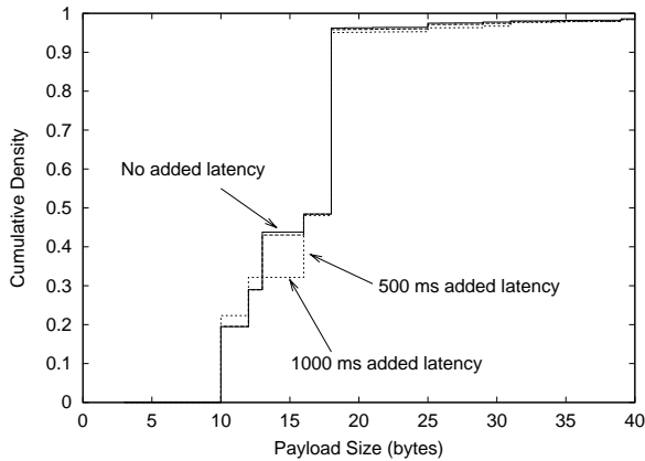
Figure 21: Age of Mythology - Payload Distributions.
