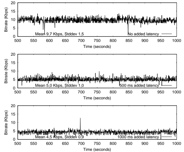
Figure 20: Command and Conquer: Generals - Bitrate versus Time.
