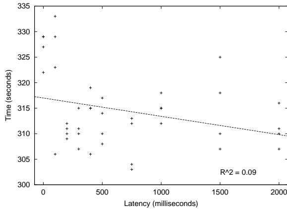
Figure 16: Command and Conquer: Generals - Explore Time versus Latency.
