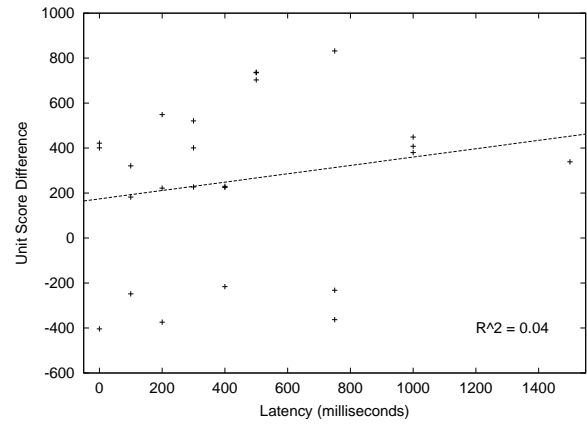
Figure 17: Age of Mythology - Unit Score Difference versus Latency.
