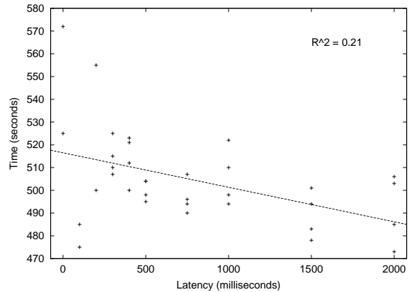
Figure 14: Command and Conquer: Generals - Build Time versus Latency.
