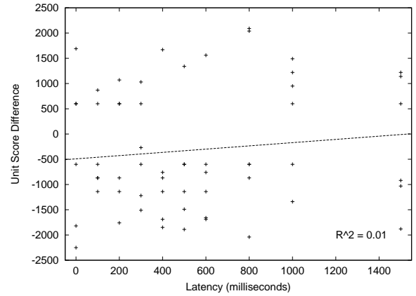
Figure 6: Warcraft III - Unit Score Difference versus Latency.
