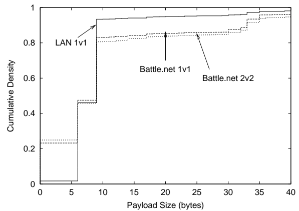
Figure 10: Warcraft III - Payload Distributions.
