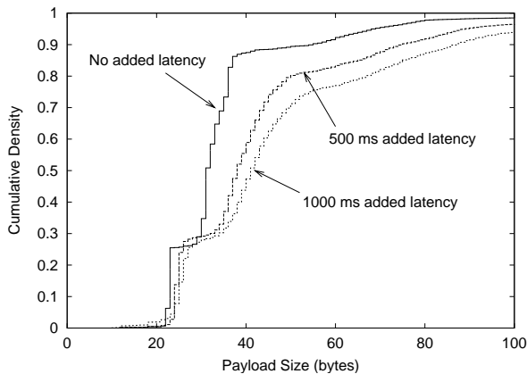
Figure 22: Command and Conquer: Generals - Payload Distributions.
