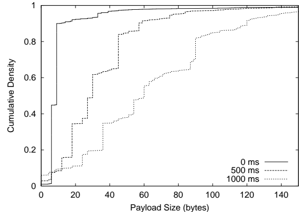
Figure 12: Warcraft III - Combat Payload Distributions.
