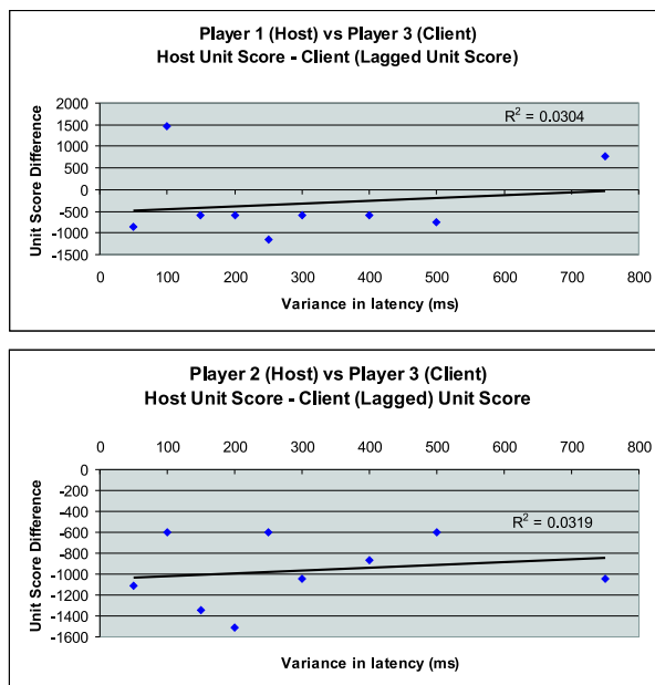
Figure 8: Warcraft III - Unit Score Difference versus Variable Latency: Player 1 versus Player 3 (top), Player 2 versus Player 3 (bottom).
