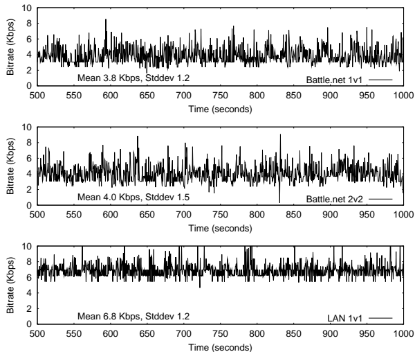
Figure 9: Warcraft III - Bitrate versus Time.
