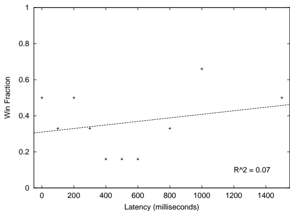
Figure 7: Warcraft III - Combat Games Won by Host (non-lagged) versus Latency (on the Client).
