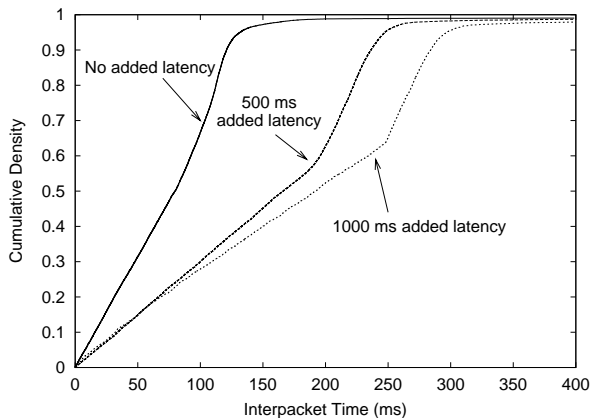
Figure 24: Command and Conquer: Generals - Inter-packet Distributions.
