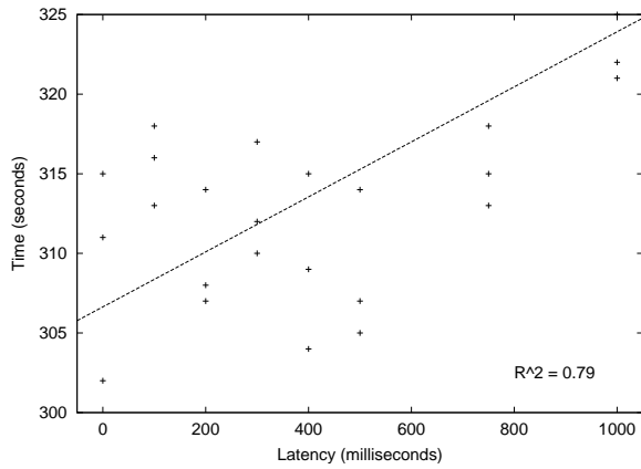
Figure 15: Age of Mythology - Explore Time versus Latency.
