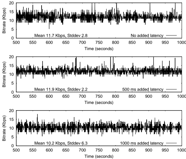
Figure 19: Age of Mythology - Bitrate versus Time.
