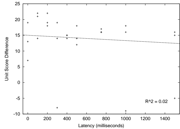
Figure 18: Command and Conquer: Generals - Unit Score Difference versus Latency.
