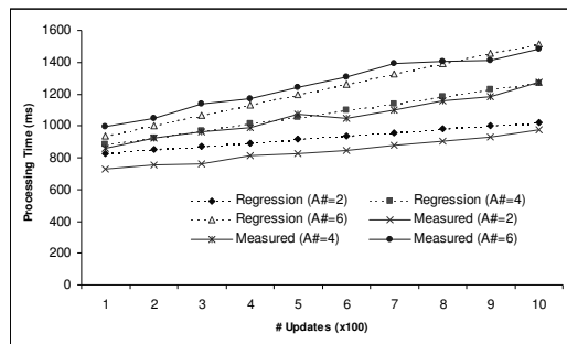
Figure 11: Cost Function Regression
