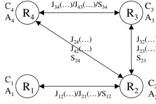
Figure 5: Extended View Definition Graph
