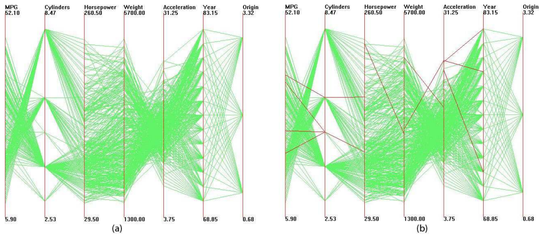
Figure 1: Parallel coordinates visualization of original Cars dataset. Outliers are highlighted with red in Fig.1-(b)
