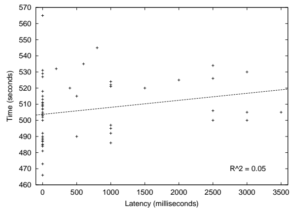
Figure 4: Warcraft III - Build Time versus Latency.
