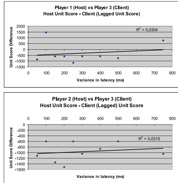
Figure 8: Warcraft III - Unit Score Difference versus Variable Latency: Player 1 versus Player 3 (top), Player 2 versus Player 3 (bottom).
