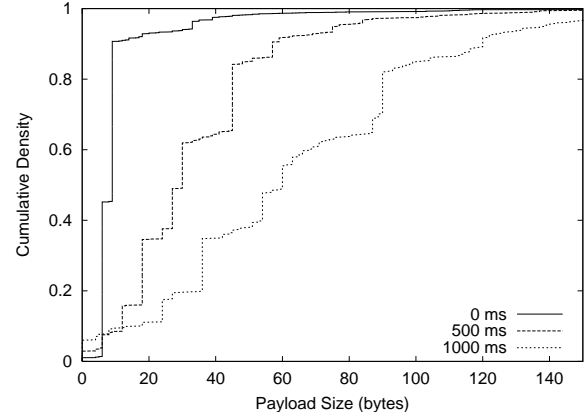
Figure 12: Warcraft III - Combat Payload Distributions.
