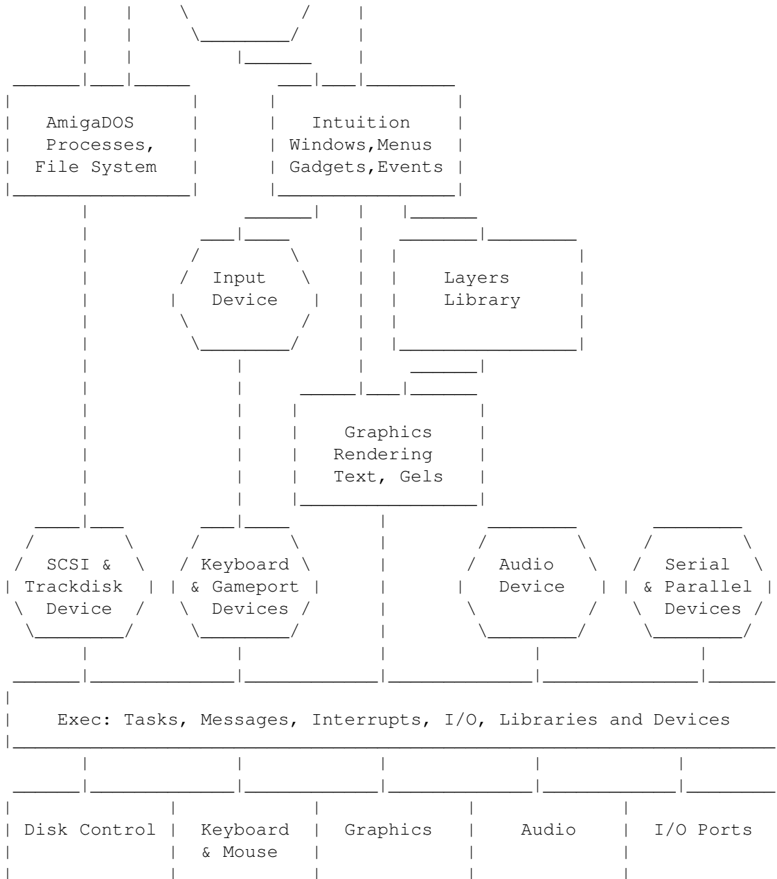
Figure 1-1: Amiga System Software Hierarchy
