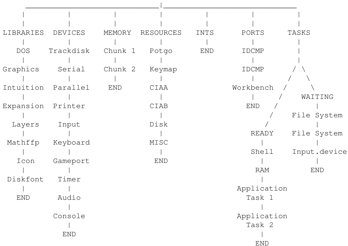
Figure 1-3: Exec and the Organization of the Amiga OS
