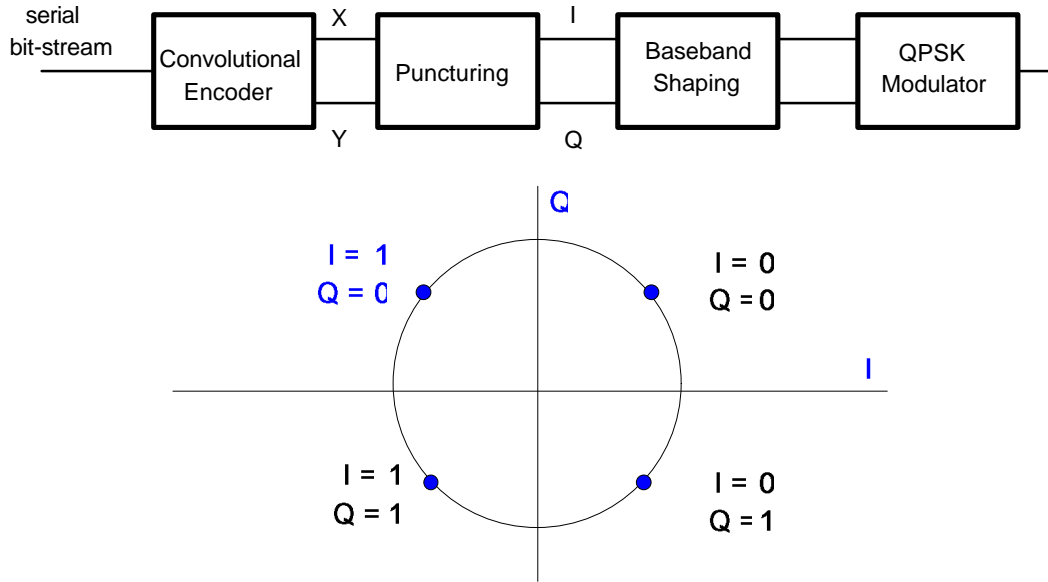
Figure 5: QPSK constellation
