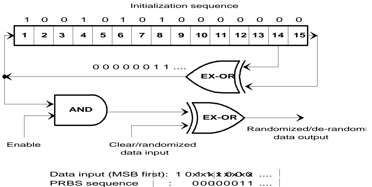
Figure 2: Randomizer/de-randomizer schematic diagram
