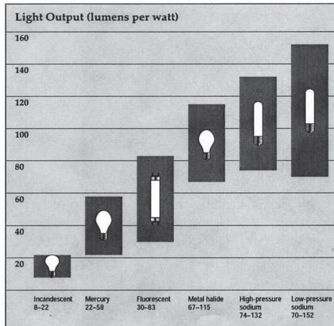
Each type of lamp differs in the amount of light it delivers per watt.
