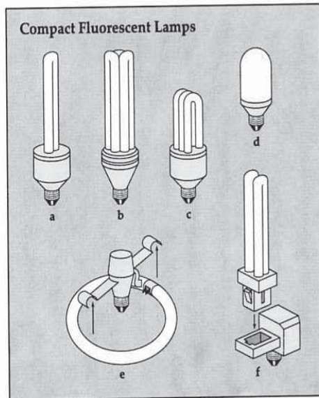
Compact fluorescent lamps (CFLs) come in a variety of sizes and shapes including (a) twin-tube integral, (b and c) triple-tube integral, (d) integral model with casing that reduces glare, (e) modular circline and ballast, and (f) modular quad-tube and ballast. CFLs can be installed in regular incandescent fixtures, and they consume less than one-third as much electricity as incandescent lamps do.
