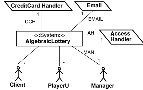
Figure 7: Algebraic Lottery: Context View version 1
