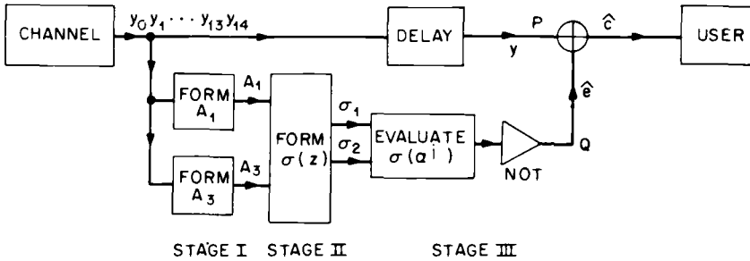
Fig. 9.5. The complete decoder.
