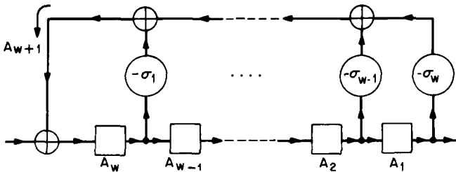
Fig. 9.4. The A_i 's are produced by a shift register.
