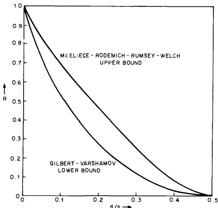
Fig. 17.7. Asymptotic bounds on the best binary codes.
