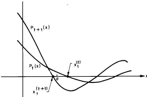
Fig. 17.5. The zeros of Krawtchouk polynomials are interlaced.
