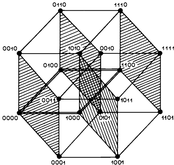
Fig. 13.6. EG(4, 2) showing the subspace S (double lines) and U_1, \dots, U_4 (shaded).
