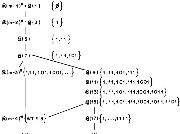
Fig. 13.5. Nesting habits of BCH and punctured RM codes.
