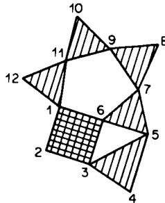
Fig. 8.4. A [12, 6, 3] code with trivial automorphism group.
