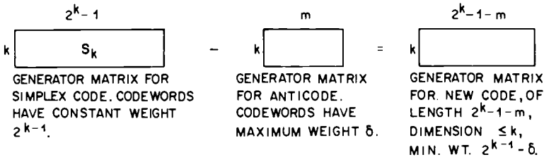
Fig. 17.1a. Using an anticode to construct new codes.
