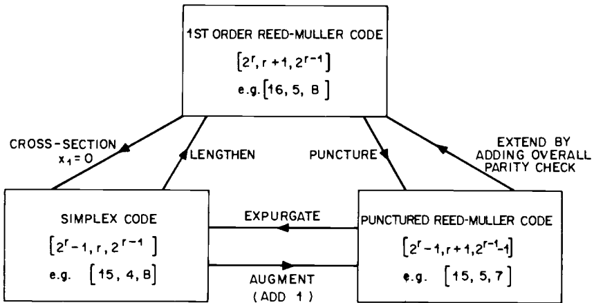
Fig. 1.13. Variations on the simplex code.
