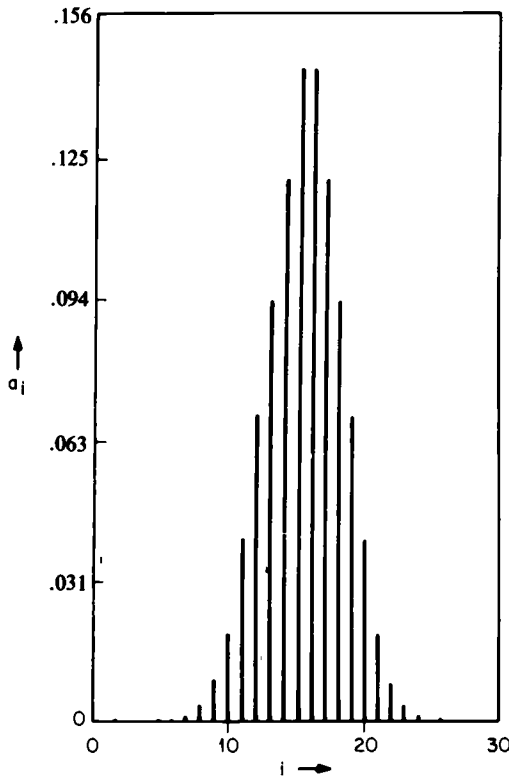
Fig. 9.7. The numbers a_i = A_i/2^{21} for the [31, 21, 5] BCH code.
