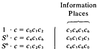
Fig. 16.10. The three permutations for permutation decoding of [7, 4, 3] code.
