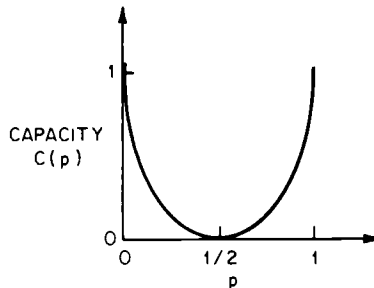
Fig. 1.9. Capacity of binary symmetric channel.
