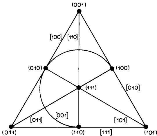
Fig. 2. The projective plane PG(2, 2) .
