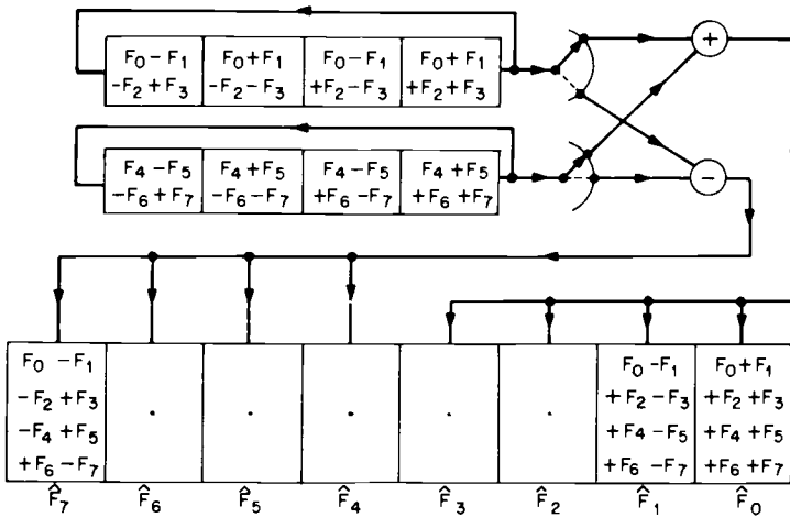
Fig. 14.11. Third stage of Green machine.
