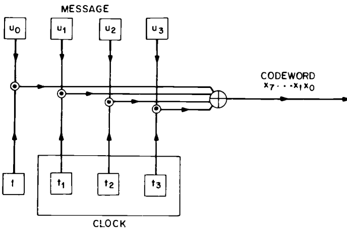
Fig. 14.8. Encoder for \mathcal{R}(1, 3) .
