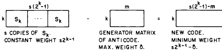
Fig. 17.1b. If the anticode has repeated columns.
