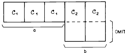
Fig. 2.6. Forming a new code by pasting together copies of two codes.
