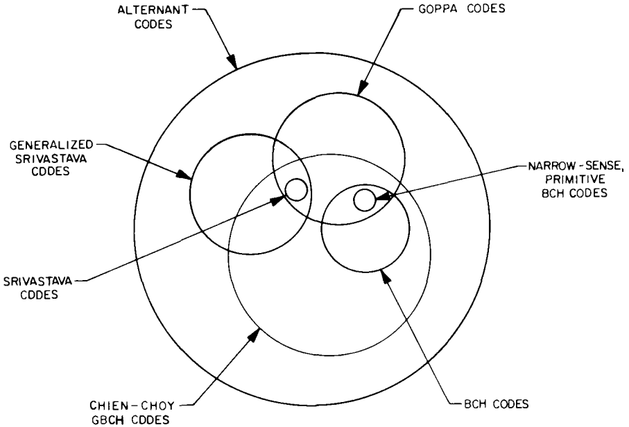
Fig. 12.1. Relationship between various subclasses of alternant codes.
