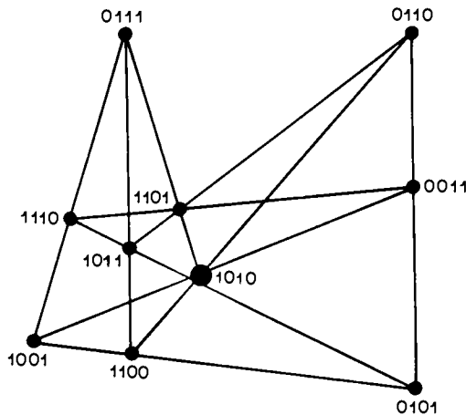
Fig. 17.3. The Desargues configuration.
