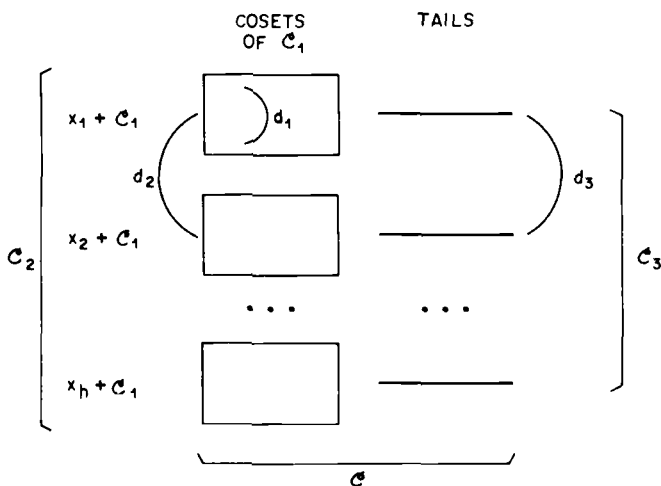
Fig. 18.4. Construction X: adding tails to \mathcal{C}_2 .
