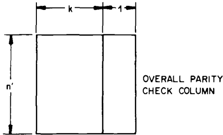
Fig. 18.6. A typical codeword of \mathcal{C} .
