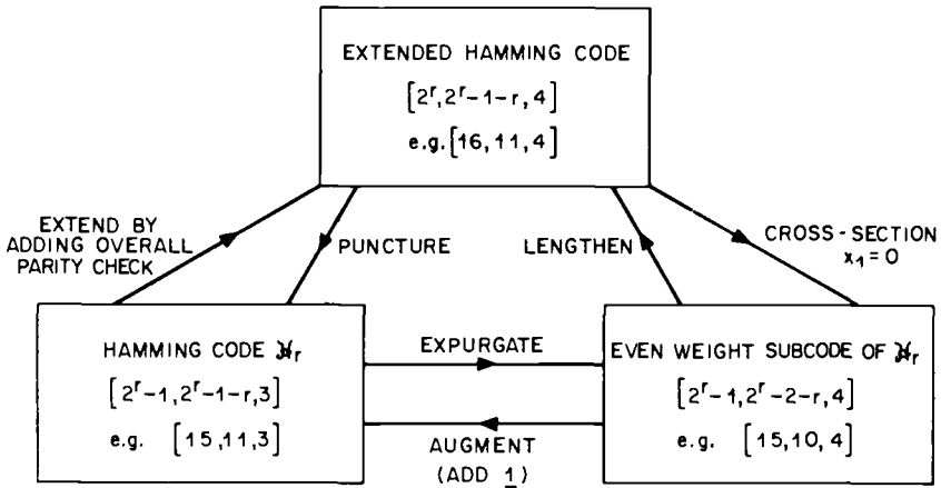
Fig. 1.11. Variations on a Hamming code.
