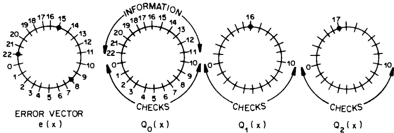
Fig. 16.11. Covering polynomials for Golay code.
