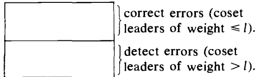
Fig. 1.8. Incomplete decoding using a standard array.
