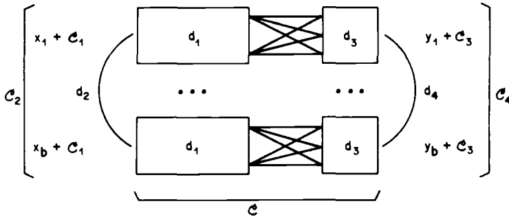
Fig. 18.5. Construction X4, combining four codes.
