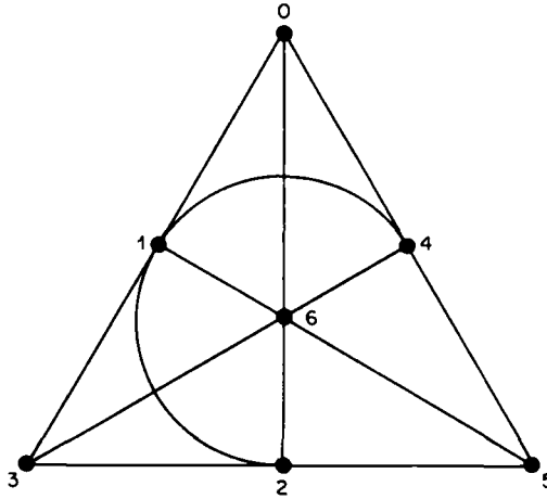
Fig. 2.12. The projective plane of order 2.
