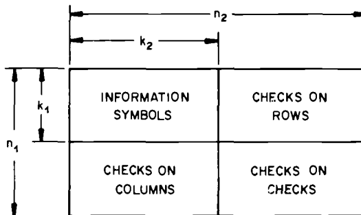
Fig. 18.1. Codewords of the direct product code \mathcal{A} \otimes \mathcal{B} .
