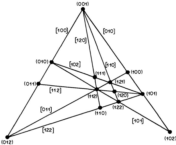
Fig. 3. The 13 points and nine of the 13 lines of the projective plane PG(2, 3) .
