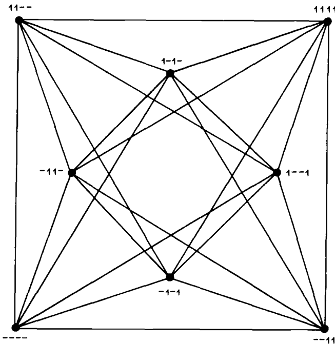
Fig. 14.5. 4-dimensional cross-polytope, with vertices corresponding to codewords of \mathcal{R}(1, 2) .
