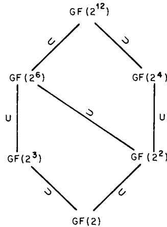
Fig. 4.3. Subfields of \text{GF}(2^{12}) .
