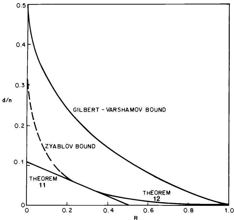
Fig. 10.10. The Justesen codes compared with the Gilbert-Varshamov bound.
