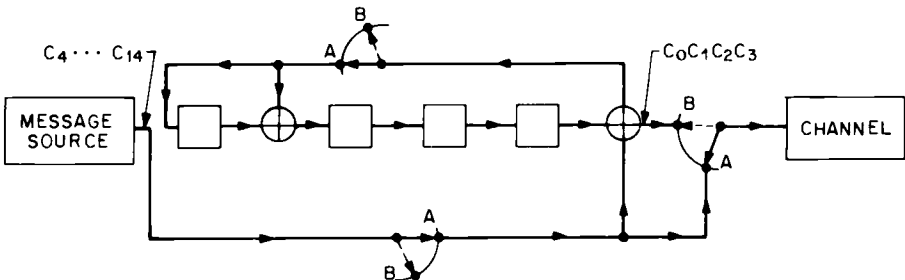
Fig. 7.9. Final version of encoder #1.
