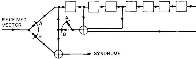
Fig. 7.12. Encoder #2 modified to calculate syndrome.
