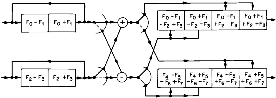
Fig. 14.10. Second stage of Green machine.
