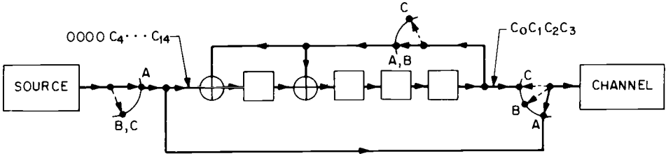
Fig. 7.7. Preliminary version of encoder #1.
