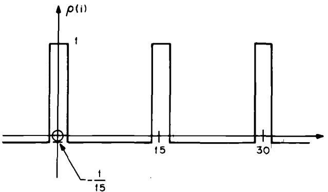
Fig. 14.4. Autocorrelation function of a PN sequence.
