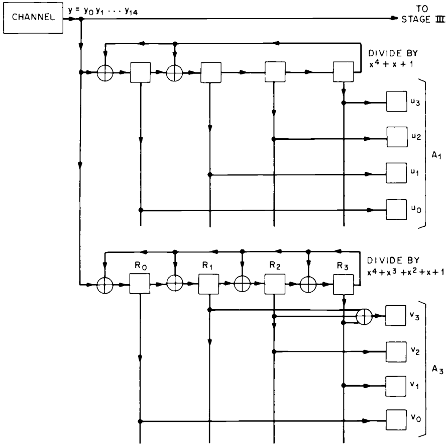
Fig. 9.3. Stage I of decoder: Finding the syndrome.
