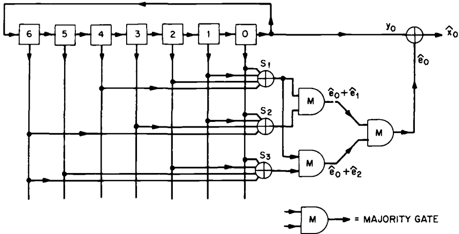
Fig. 13.8. Two-step majority decoding of the [7, 4, 3] code.
