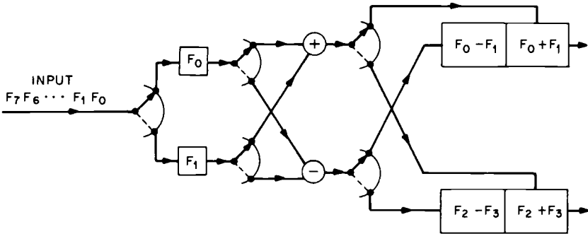
Fig. 14.9. First stage of Green machine.
