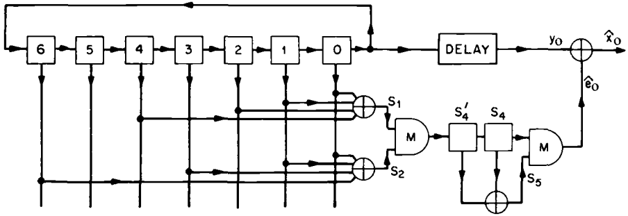
Fig. 13.9. Decoder for [7, 4, 3] code using sequential code reduction.
