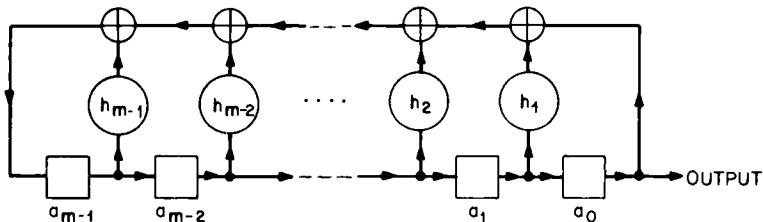
Fig. 14.2. Feedback shift register defined by h(x) .
