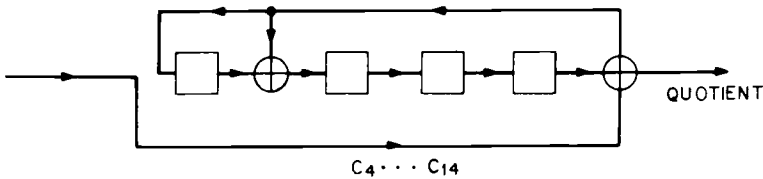
Fig. 7.8. Division circuit, with premultiplication by x^4 .
