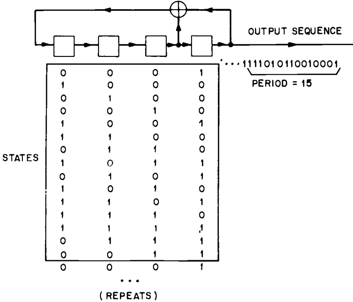
Fig. 14.3. Shift register corresponding to h(x) = x^4 + x + 1 , showing successive states.
