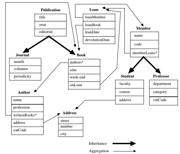
FIG. 1. FacultyLibrary example schema.
