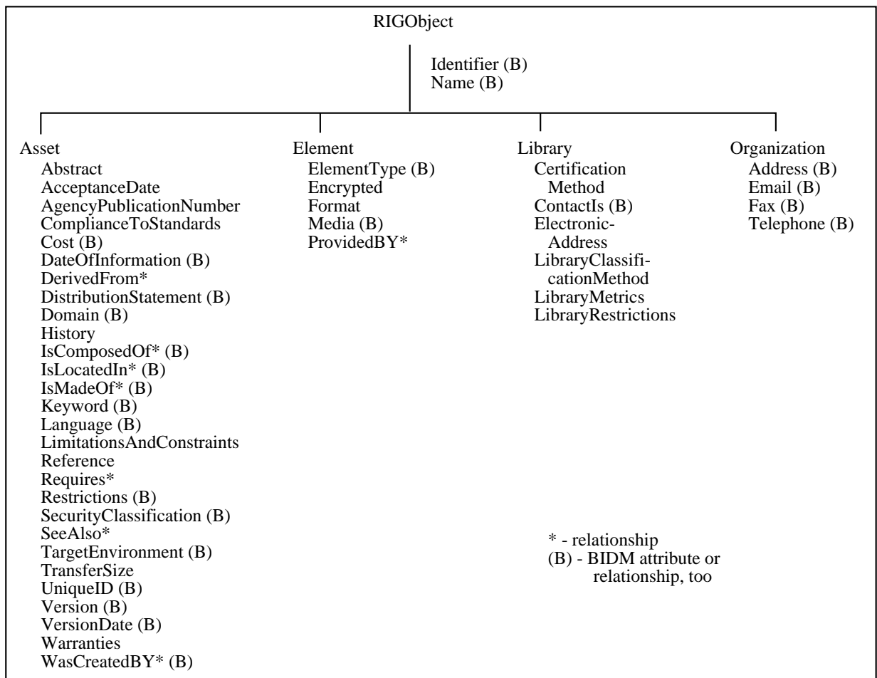
Figure 1: UDM Class Hierarchy
