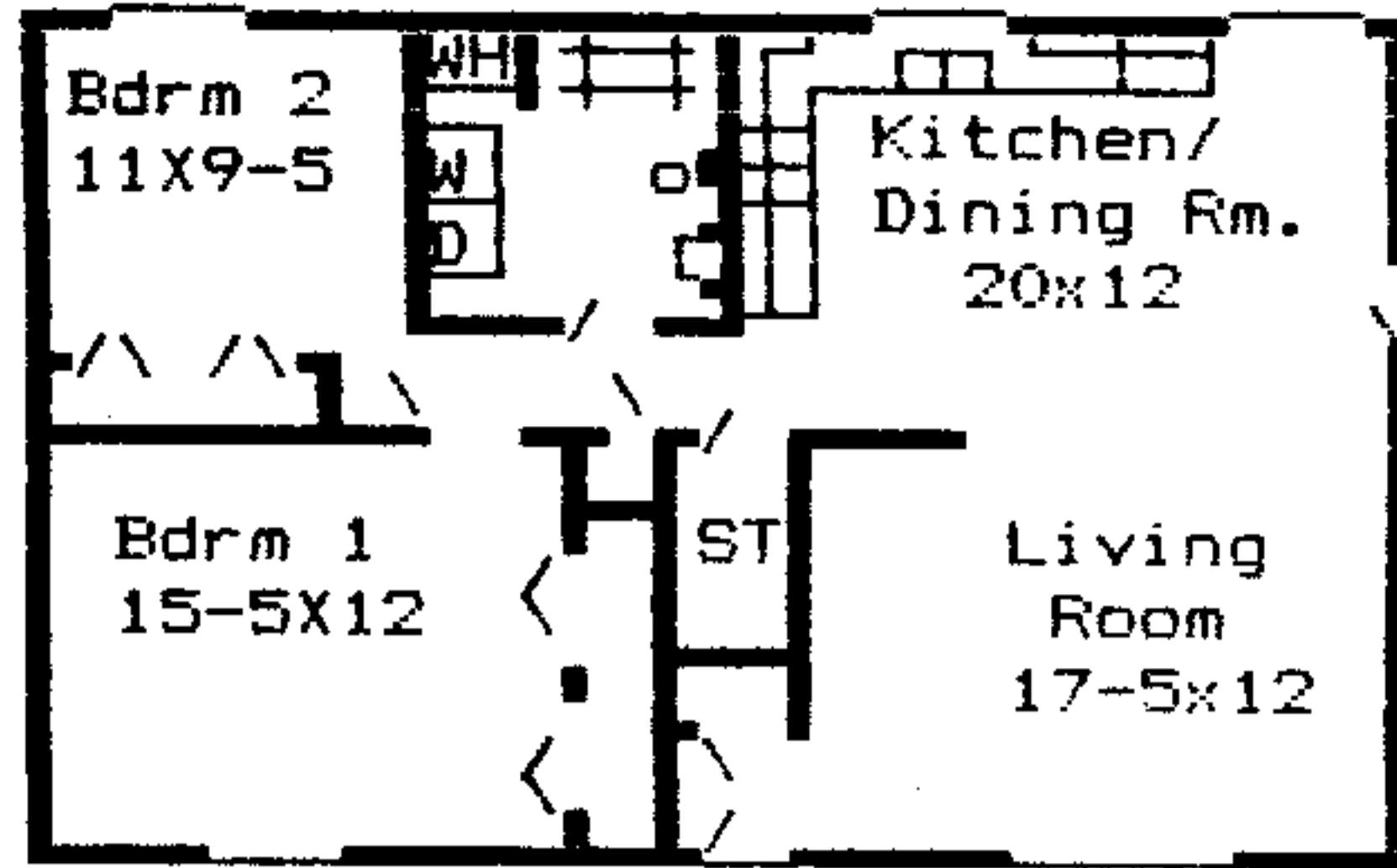
Fig. 1—Computer aided floor plan design incorporating graphic symbols and upper and lower-case alphanumerics.
