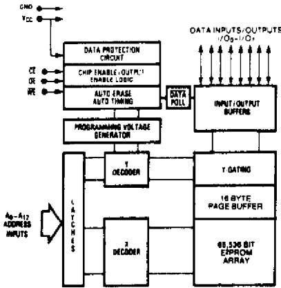
2864A Functional Block Diagram
