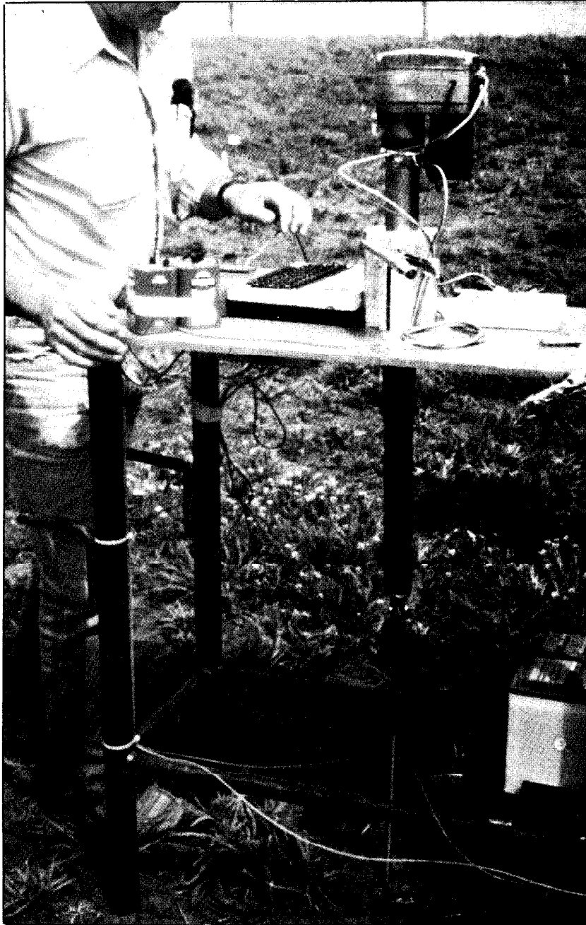
Kansas State University researcher uses a Model 100/analog-to-digital converter unit to monitor soil permeability.
