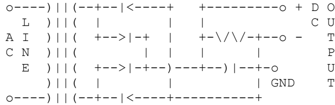
A power supply consisting of a full wave rectifier circuit feeding a capacitor input filter circuit
