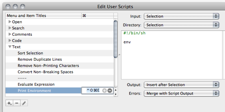
Figure 8-3 Adding a shell script
