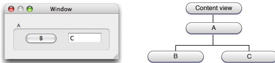
Figure 3-1 View hierarchy
