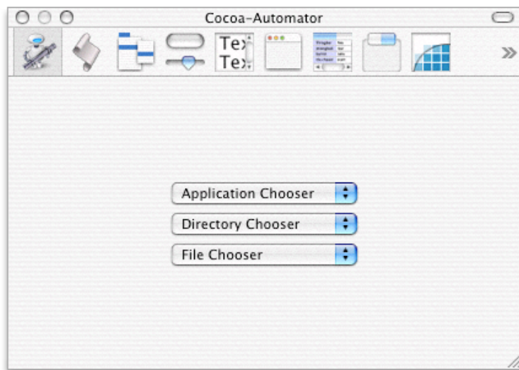
Figure 4 Cocoa-Automator palette
