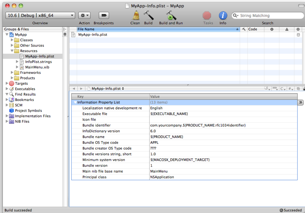
Figure 1 Editing the information property list in Xcode
