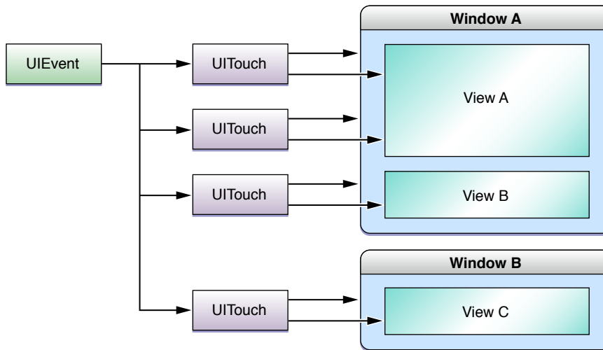
Figure 2-3 All touches for a given touch event
