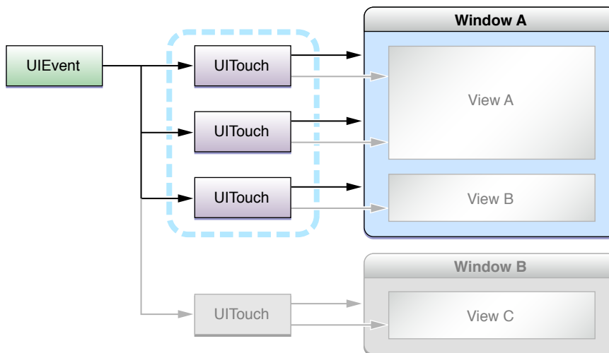
Figure 2-4 All touches belonging to a specific window
