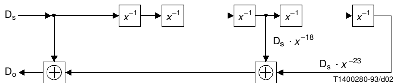
FIGURE 2/V.38 Descrambler
