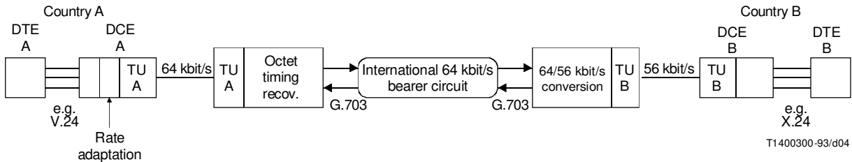
FIGURE II.1/V.38
