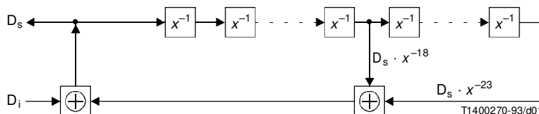
FIGURE 1/V.38 Scrambler
