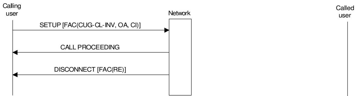
FIGURE 1-3/Q.955
