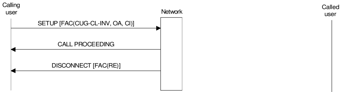
FIGURE 1-2/Q.955
