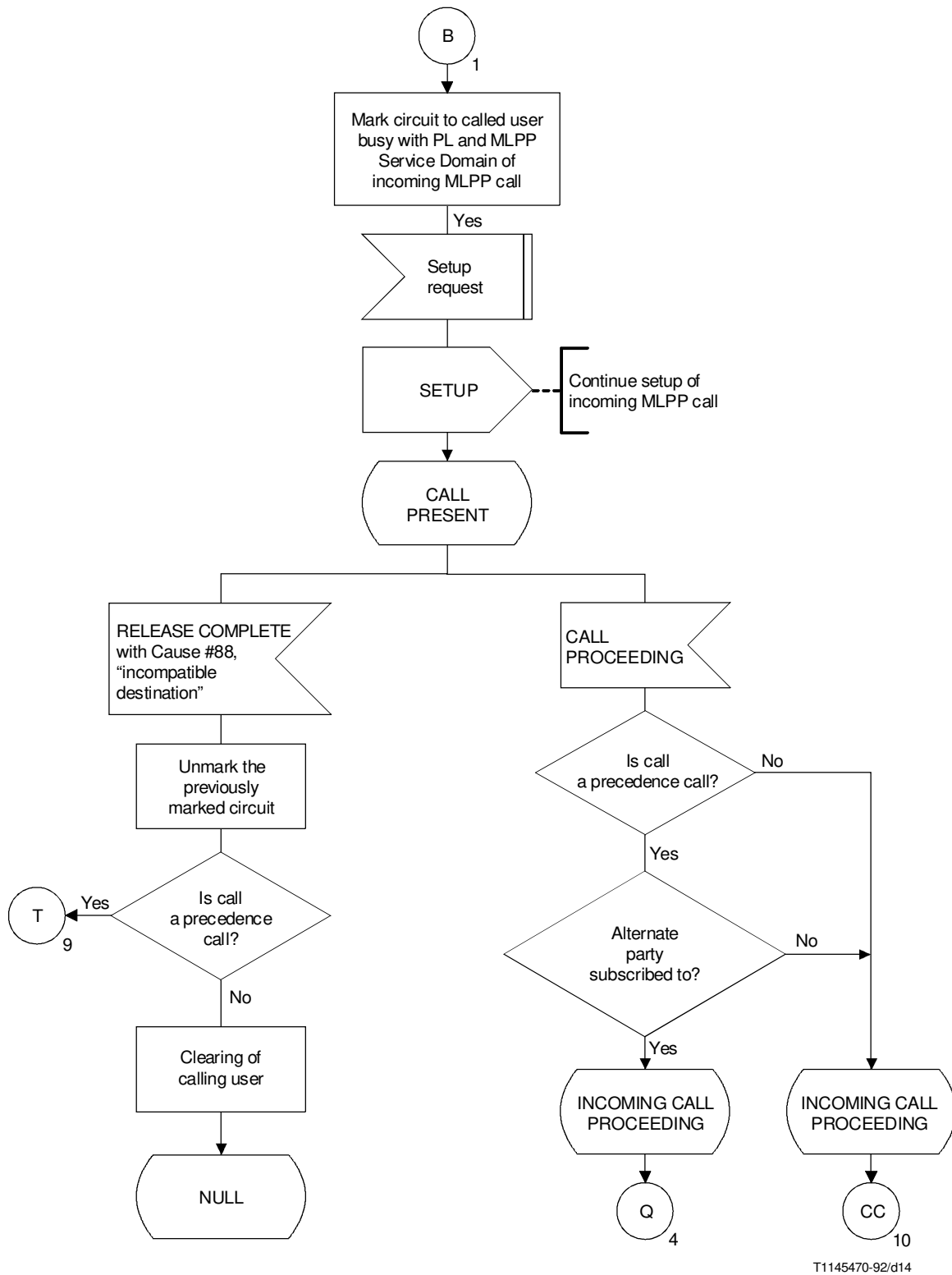
FIGURE 3-11/Q.955 (Sheet 2 of 14)
