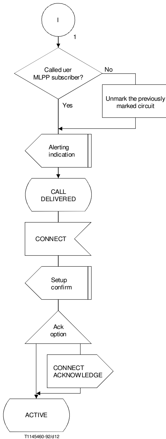
FIGURE 3-10/Q.955 (Sheet 2 of 2) Calling User – Procedure without DSS 1 LFB query (procedure for outgoing MLPP call)
