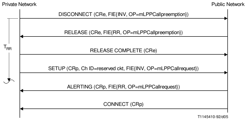
FIGURE 3-5/Q.955 Normal operation for MLPP without LFB option (originating private ISDN – successful preemption)
