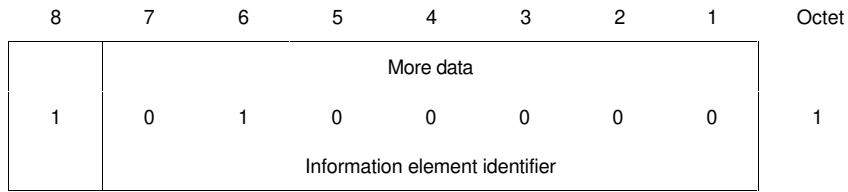
FIGURE 4-26/Q.931 More data information element
