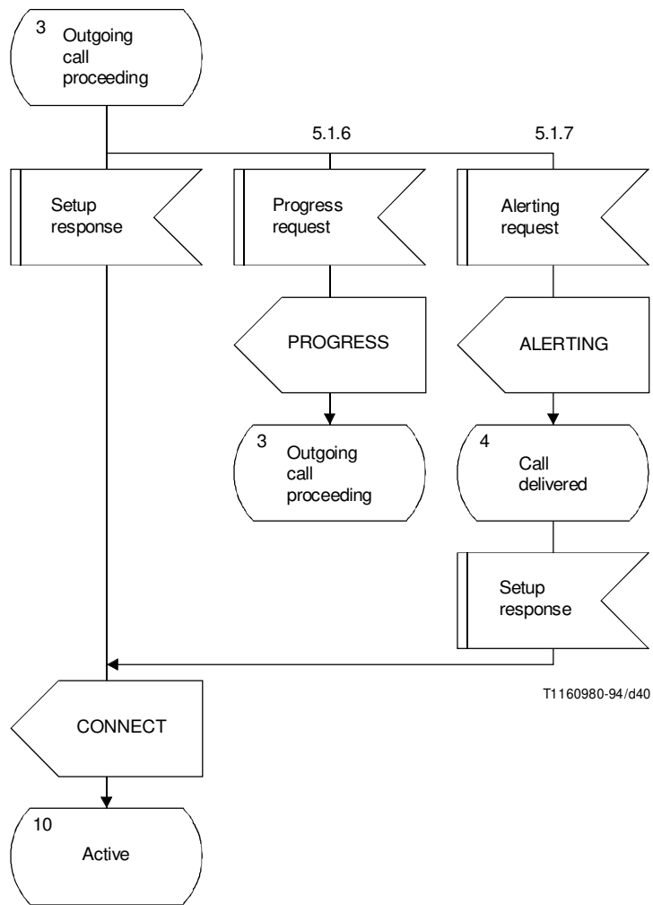
a) Outgoing set-up procedure (2 of 2)
