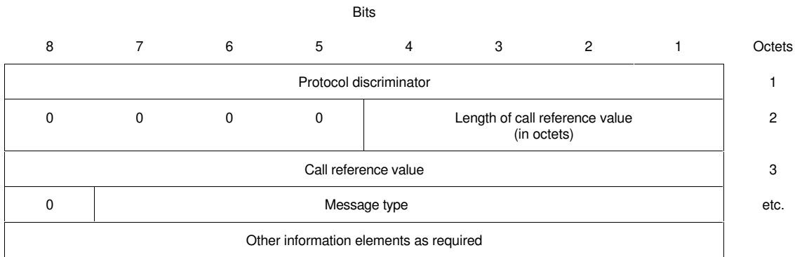
FIGURE 4-1/Q.931 General message organization example
