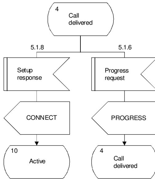
FIGURE A.6/Q.931 (Sheet 7 of 27) Detailed protocol control (network side) point-point
