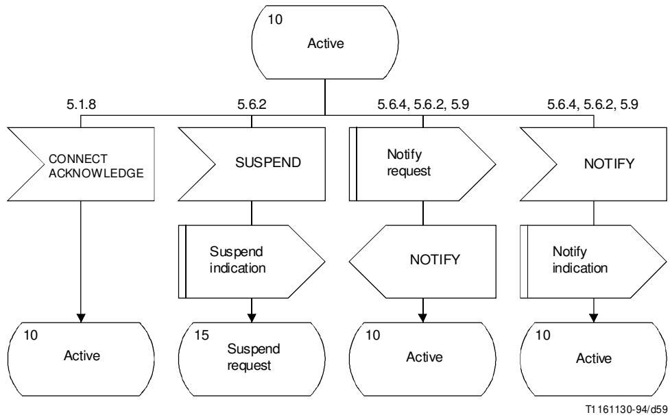
FIGURE A.6/Q.931 (Sheet 13 of 27) Detailed protocol control (network side) point-point
