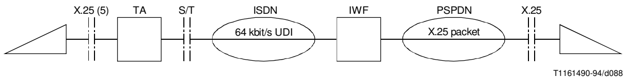
FIGURE I.4/Q.931 BC = 64 kbit/s UDI – Packet application → PSPDN
