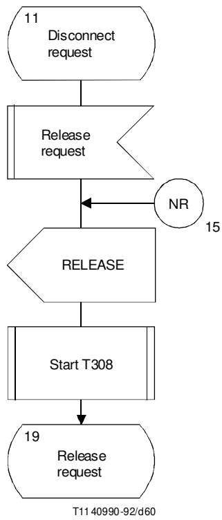
FIGURE A.6/Q.931 (Sheet 14 of 27) Detailed protocol control (network side) point-point
