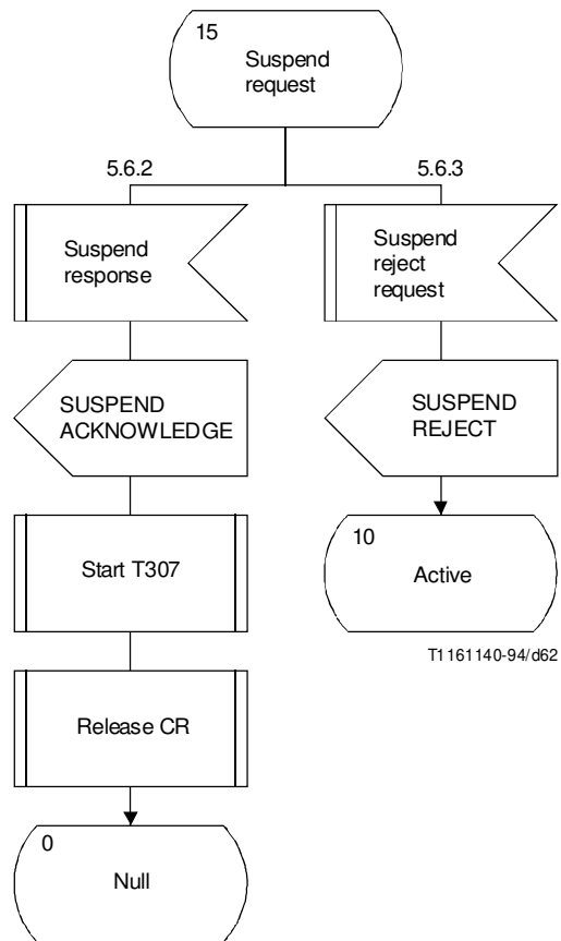
FIGURE A.6/Q.931 (Sheet 16 of 27) Detailed protocol control (network side) point-point
