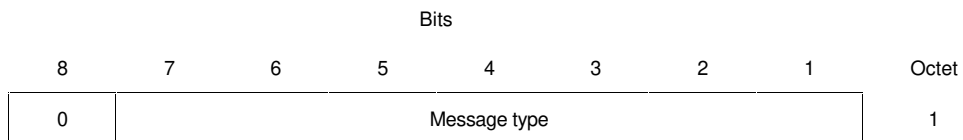
FIGURE 4-6/Q.931 Message type
