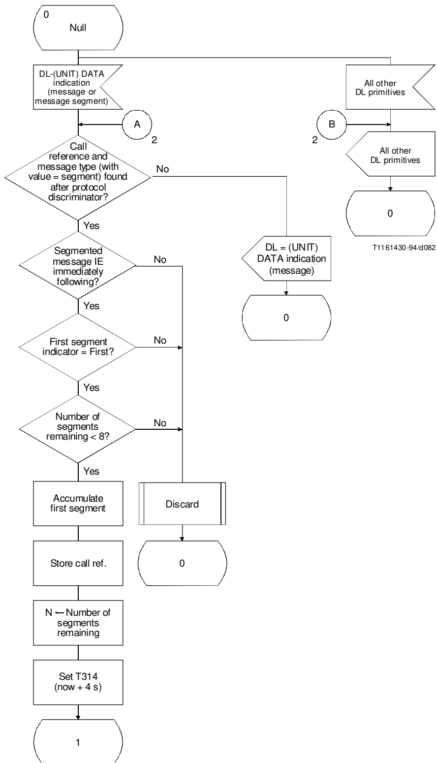
FIGURE H.5/Q.931 (Sheet 1 of 3) Message Reassembler SDL
