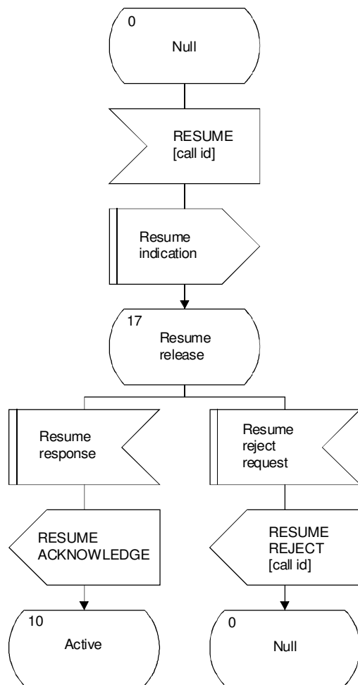
d) Resume procedure
