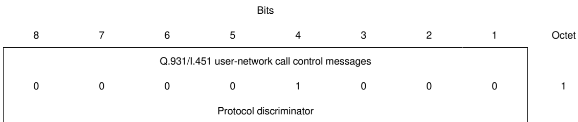
FIGURE 4-2/Q.931 Protocol discriminator
