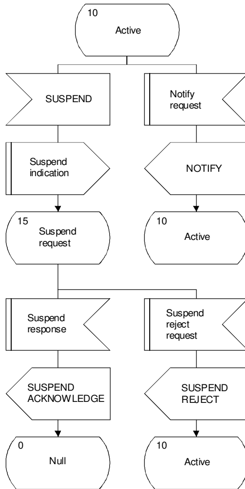
e) Suspend procedure
