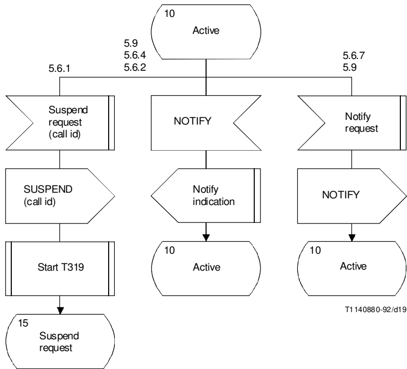
FIGURE A.3/Q.931 (Sheet 10 of 25) Detailed protocol control (user side)
