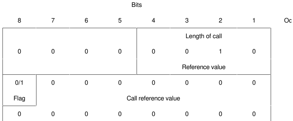
b) Two octet call reference value
