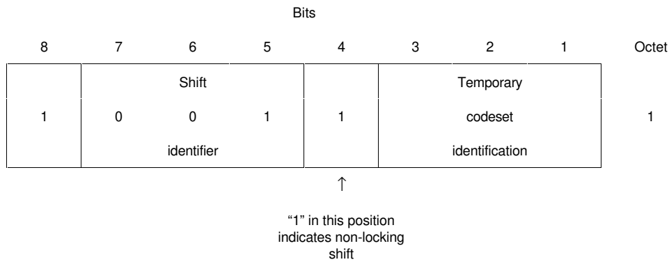
FIGURE 4-10/Q.931 Non-locking Shift information element
