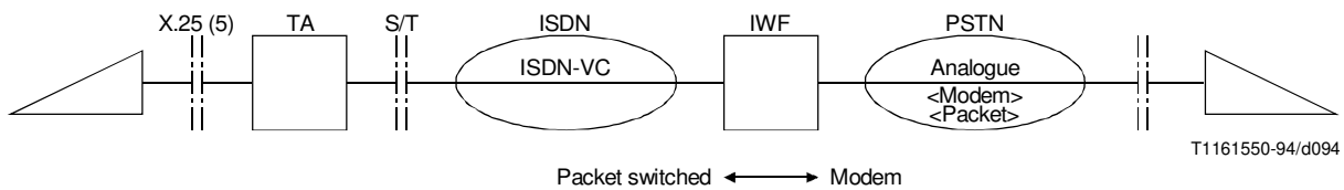
FIGURE I.10/Q.931 BC = ISDN virtual circuit (VC) → PSTN
