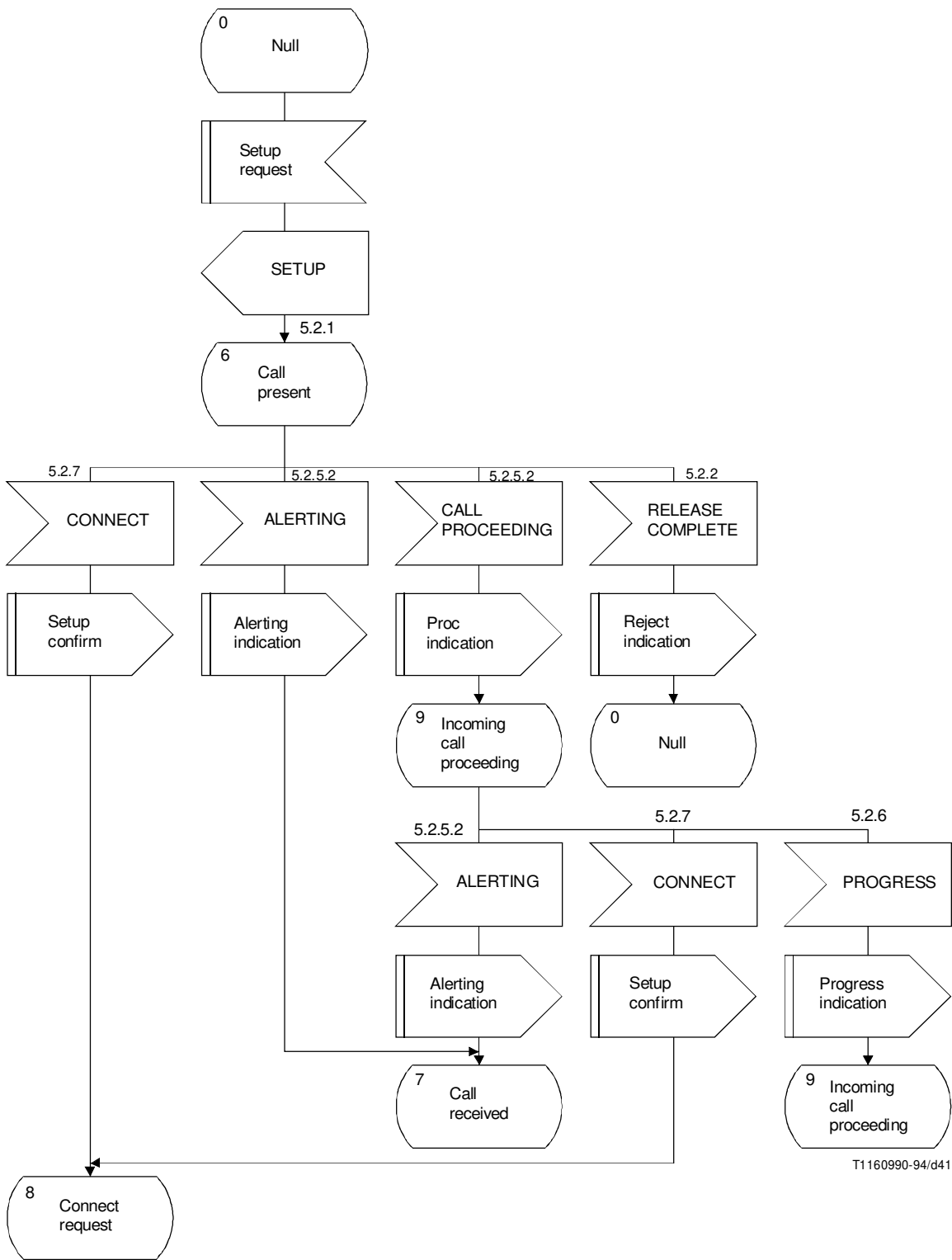
b) Incoming set-up procedure (1 of 2)
