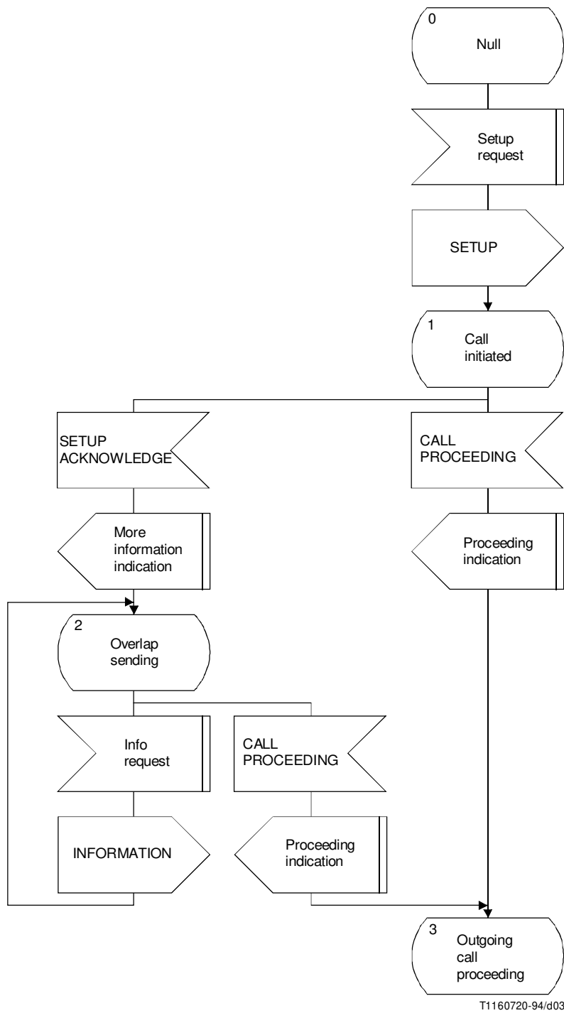
a) Outgoing set-up procedure (1 of 2)
