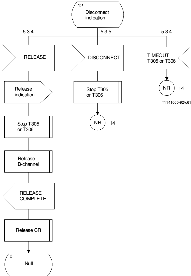
FIGURE A.6/Q.931 (Sheet 15 of 27) Detailed protocol control (network side) point-point
