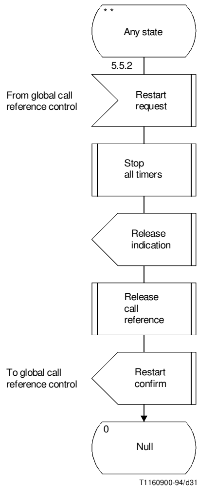
FIGURE A.3/Q.931 (Sheet 22 of 25) Detailed protocol control (user side)
