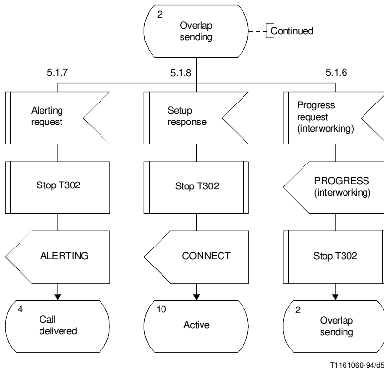
FIGURE A.6/Q.931 (Sheet 5 of 27) Detailed protocol control (network side) point-point
