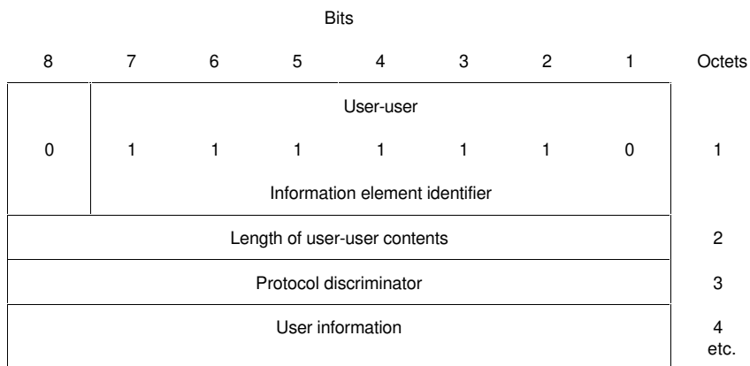
FIGURE 4-36/Q.931
