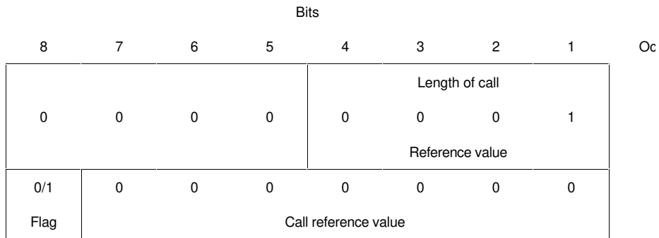
a) One octet call reference value
