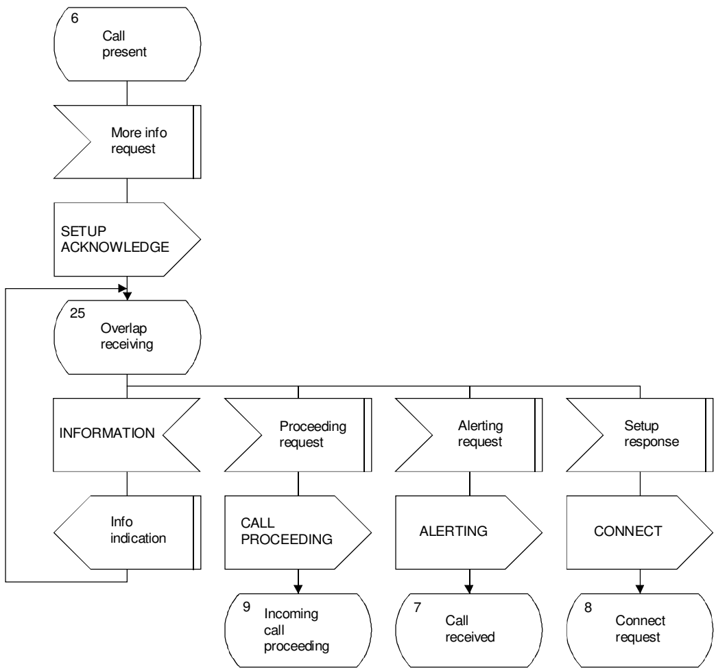
c) Overlap receiving procedure
