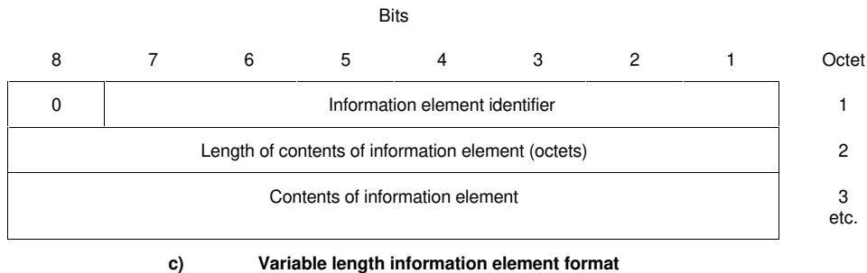
FIGURE 4-7/Q.931
