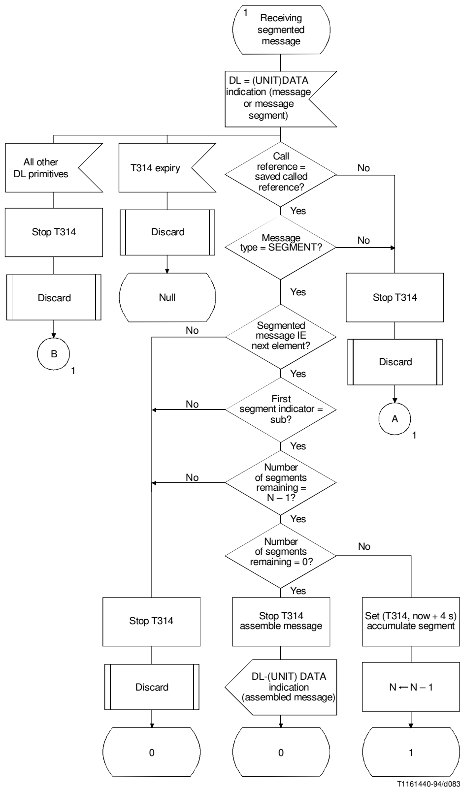
FIGURE H.5/Q.931 (Sheet 2 of 3) Message Reassembler SDL
