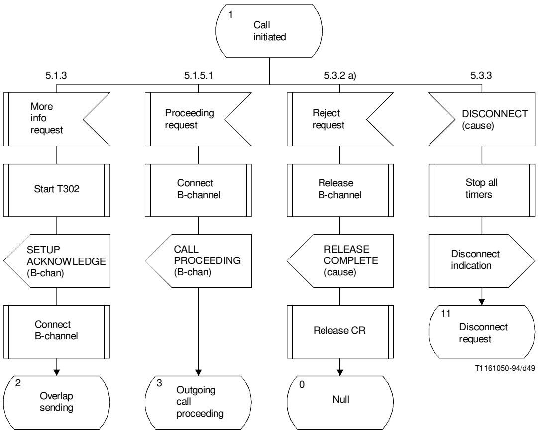
FIGURE A.6/Q.931 (Sheet 3 of 27) Detailed protocol control (network side) point-point
