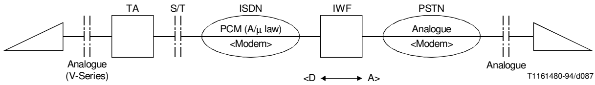
FIGURE I.3/Q.931 BC = 3.1 kHz audio – Voice → PSTN
