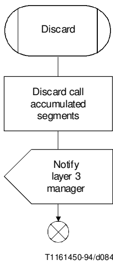
FIGURE H.5/Q.931 (Sheet 3 of 3) Message Reassembler SDL
