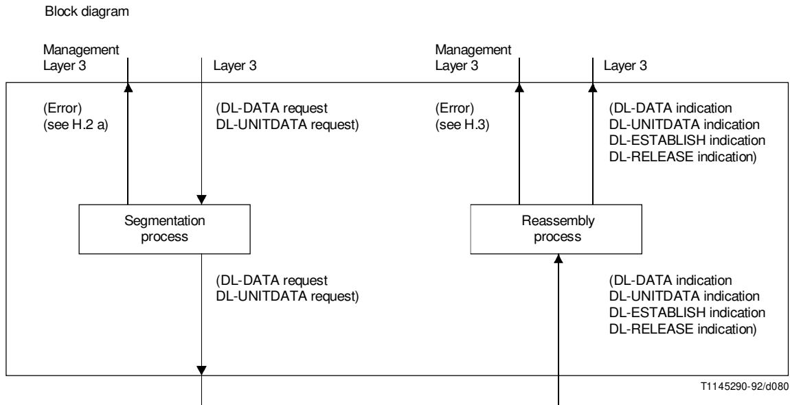
FIGURE H.3/Q.931 Segmentation Functional Interaction Diagram
