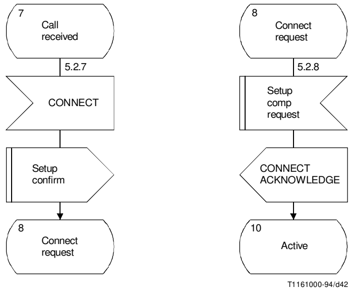
b) Incoming set-up procedure (2 of 2)
