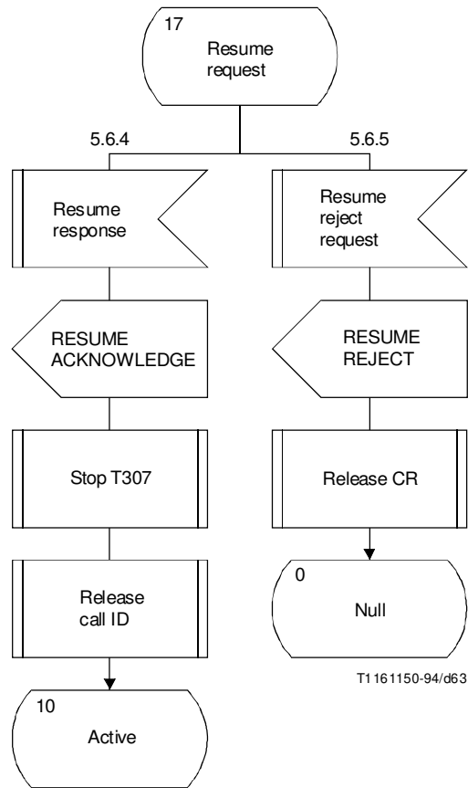
FIGURE A.6/Q.931 (Sheet 17 of 27) Detailed protocol control (network side) point-point
