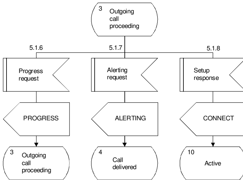
FIGURE A.6/Q.931 (Sheet 6 of 27) Detailed protocol control (network side) point-point
