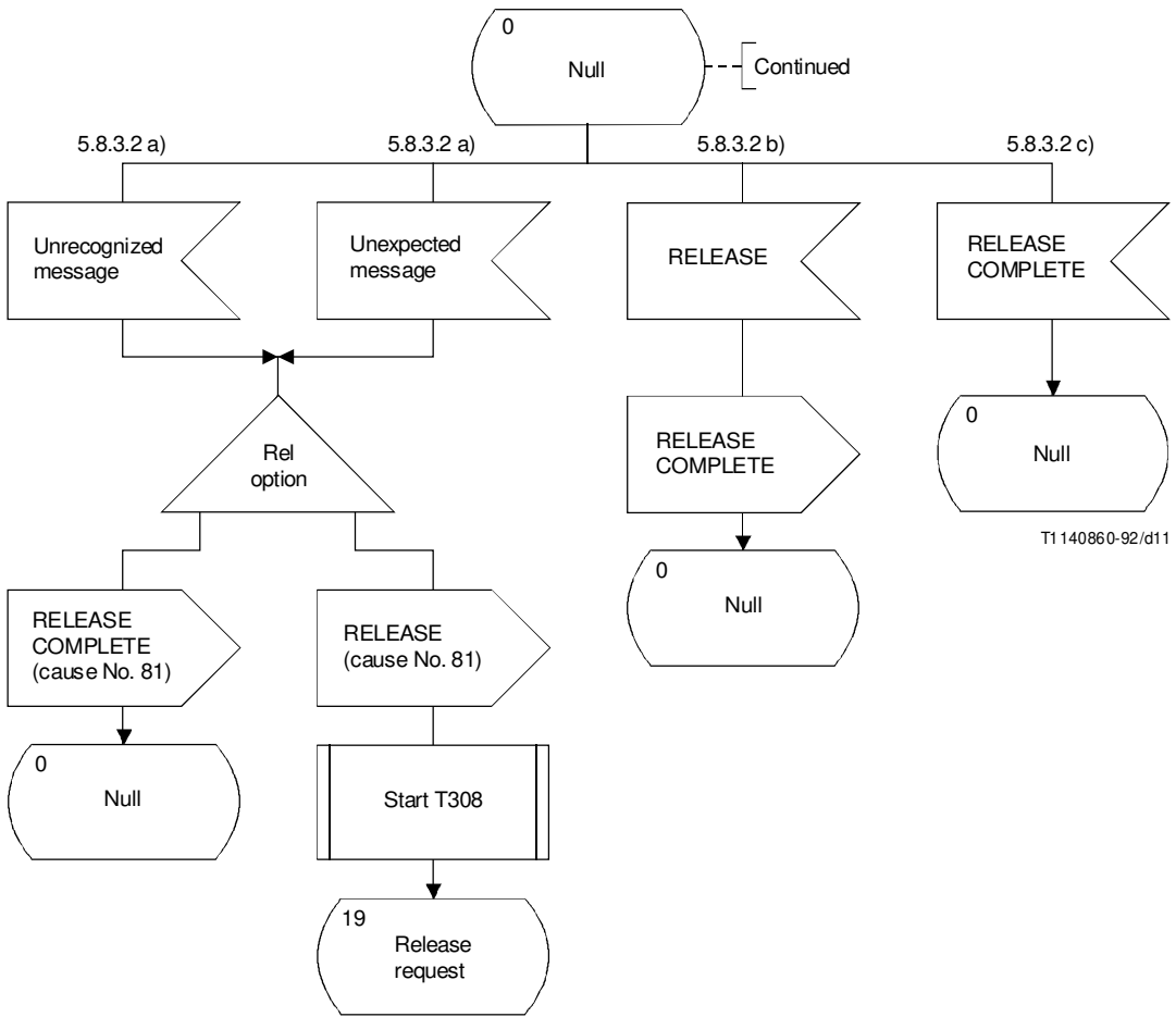
FIGURE A.3/Q.931 (Sheet 2 of 25) Detailed protocol control (user side)
