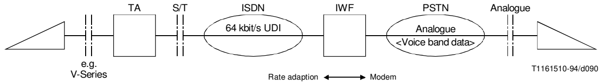
FIGURE I.6/Q.931
