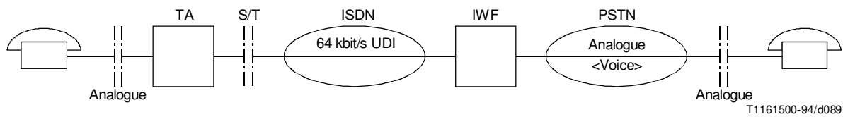
FIGURE I.5/Q.931
