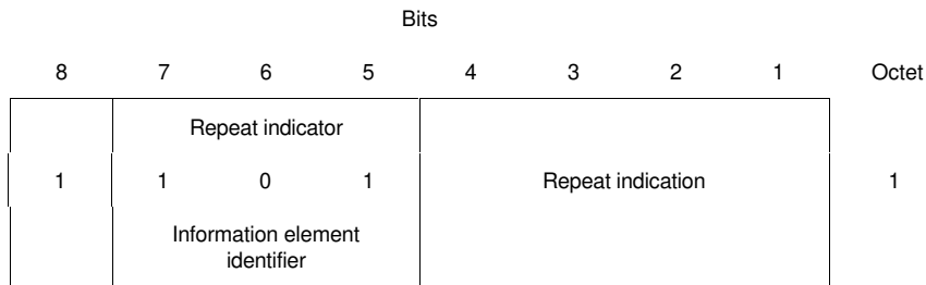
FIGURE 4-30/Q.931
