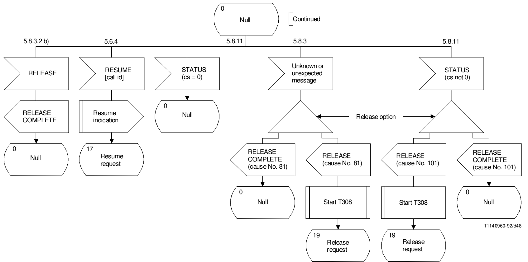
FIGURE A.6/Q.931 (Sheet 2 of 27) Detailed protocol control (network side) point-point
