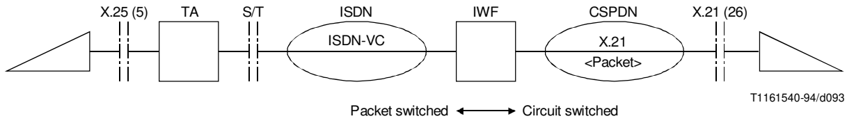
FIGURE I.9/Q.931 BC = ISDN virtual circuit (VC) → CSPDN
