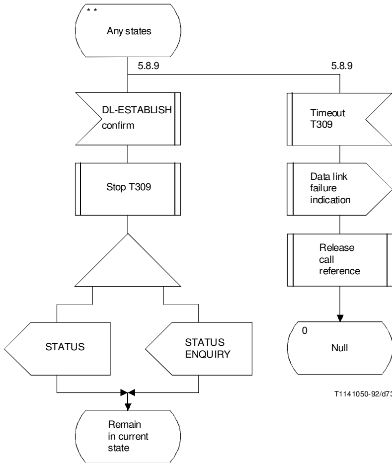
FIGURE A.6/A.931 (Sheet 27 of 27) Detailed protocol control (network side) point-point
