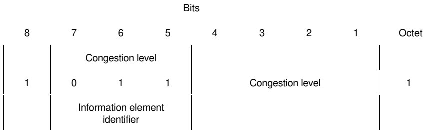
FIGURE 4-20/Q.931 Congestion level information element
