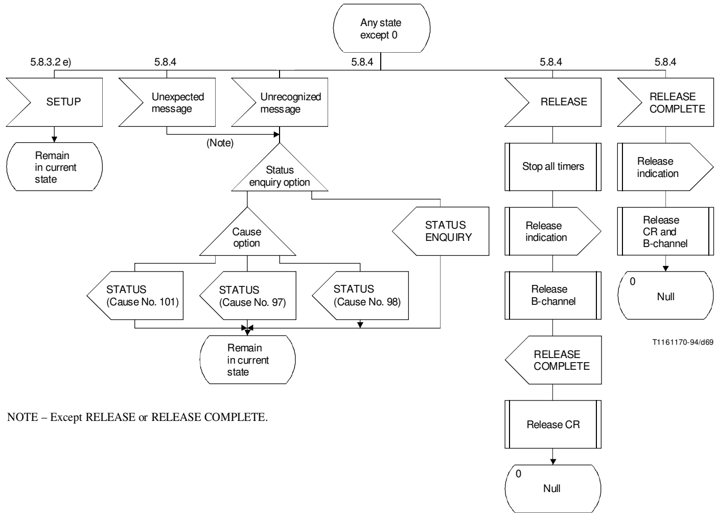
a) Error handling SDL diagram (1 of 2)
