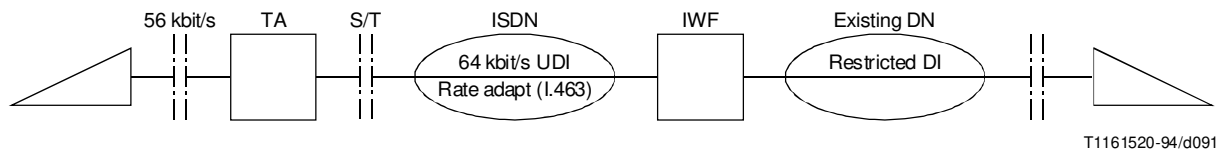
FIGURE I.7/Q.931
