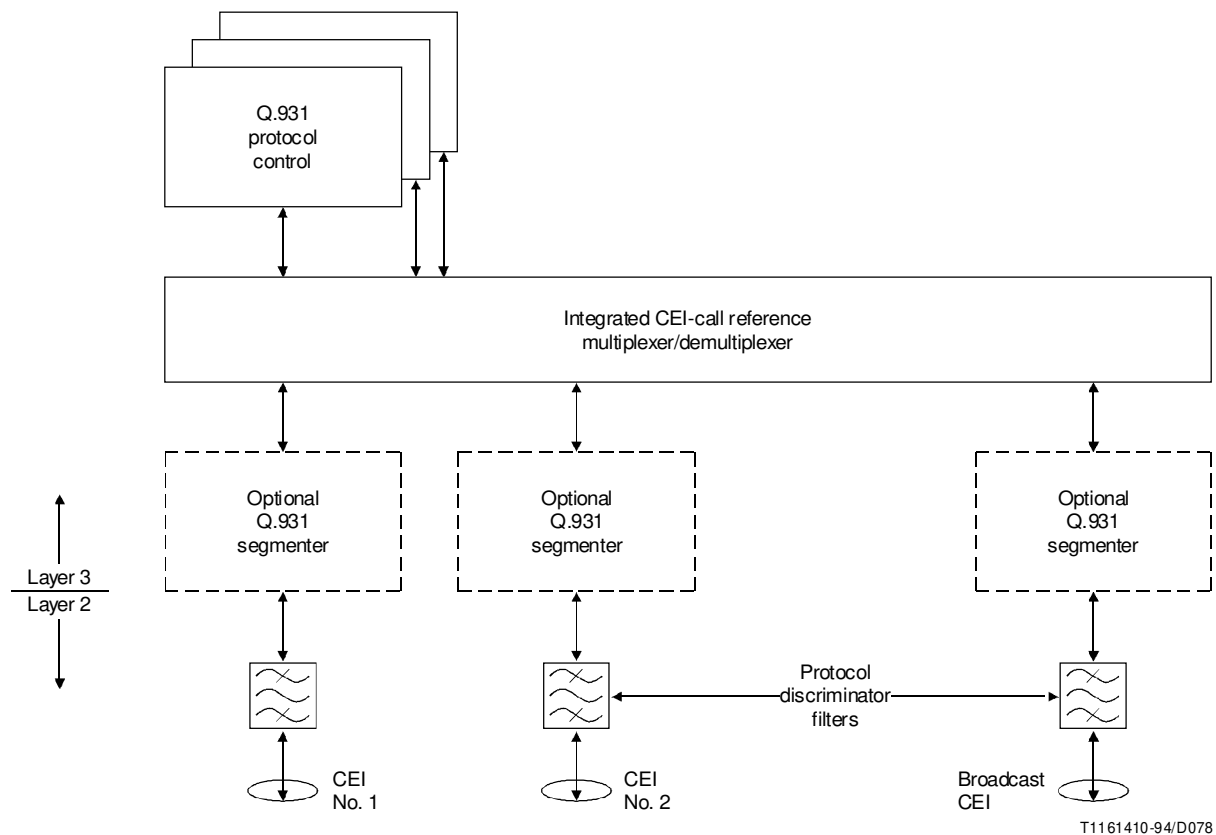
FIGURE H.1/Q.931
