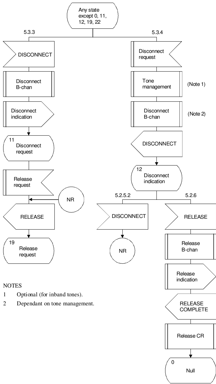
c) Clearing procedure (1 of 2)
