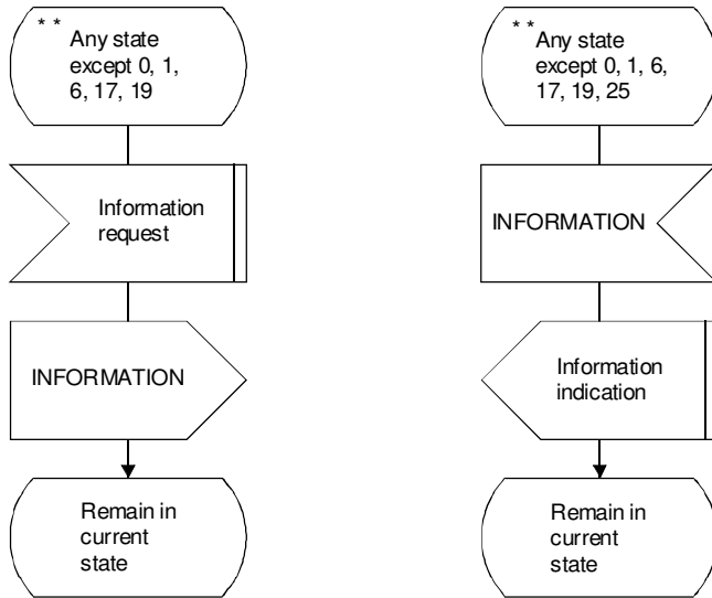
FIGURE A.3/Q.931 (Sheet 18 of 25) Detailed protocol control (user side)
