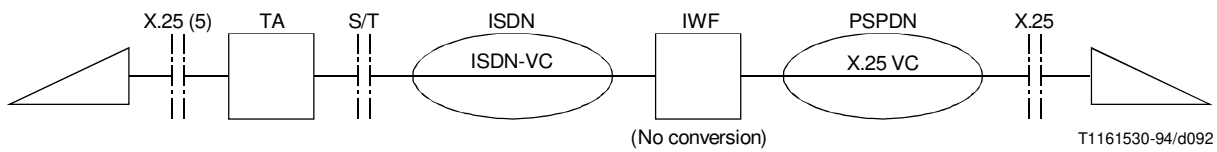
FIGURE I.8/Q.931 BC = ISDN virtual circuit (VC) → PSPDN
