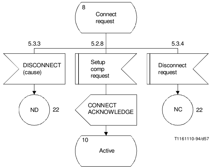
FIGURE A.6/Q.931 (Sheet 11 of 27) Detailed protocol control (network side) point-point
