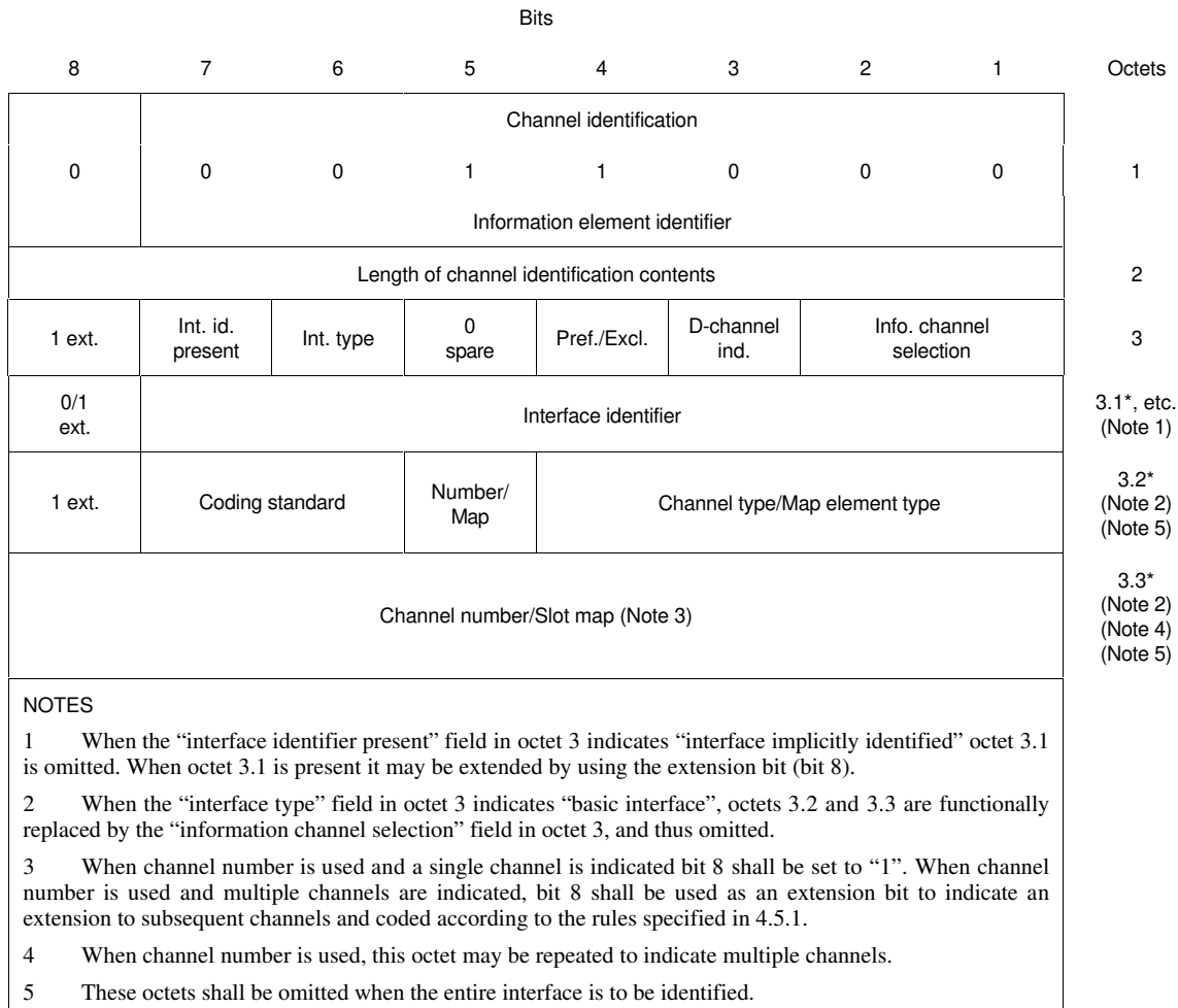
FIGURE 4-18/Q.931
