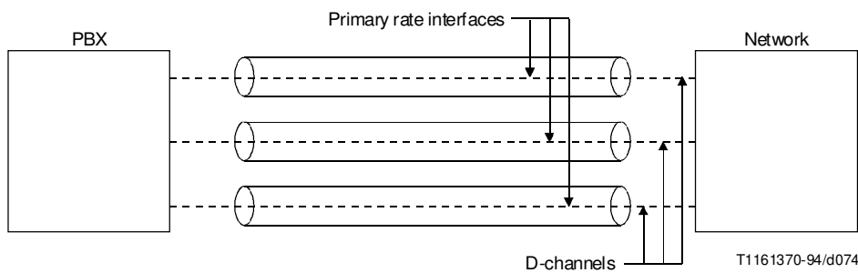
FIGURE F.1/Q.931
