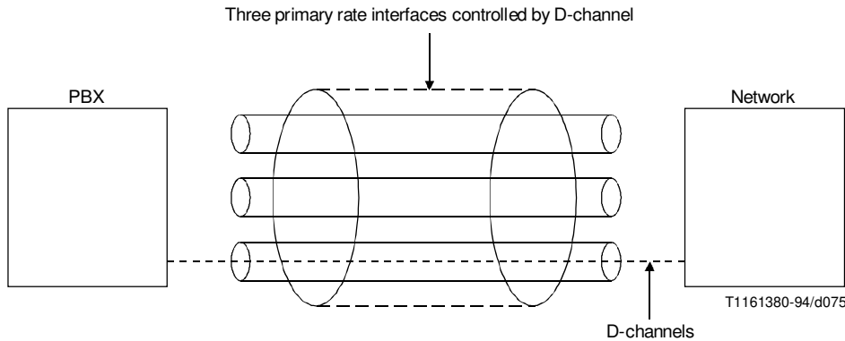
FIGURE F.2/Q.931
