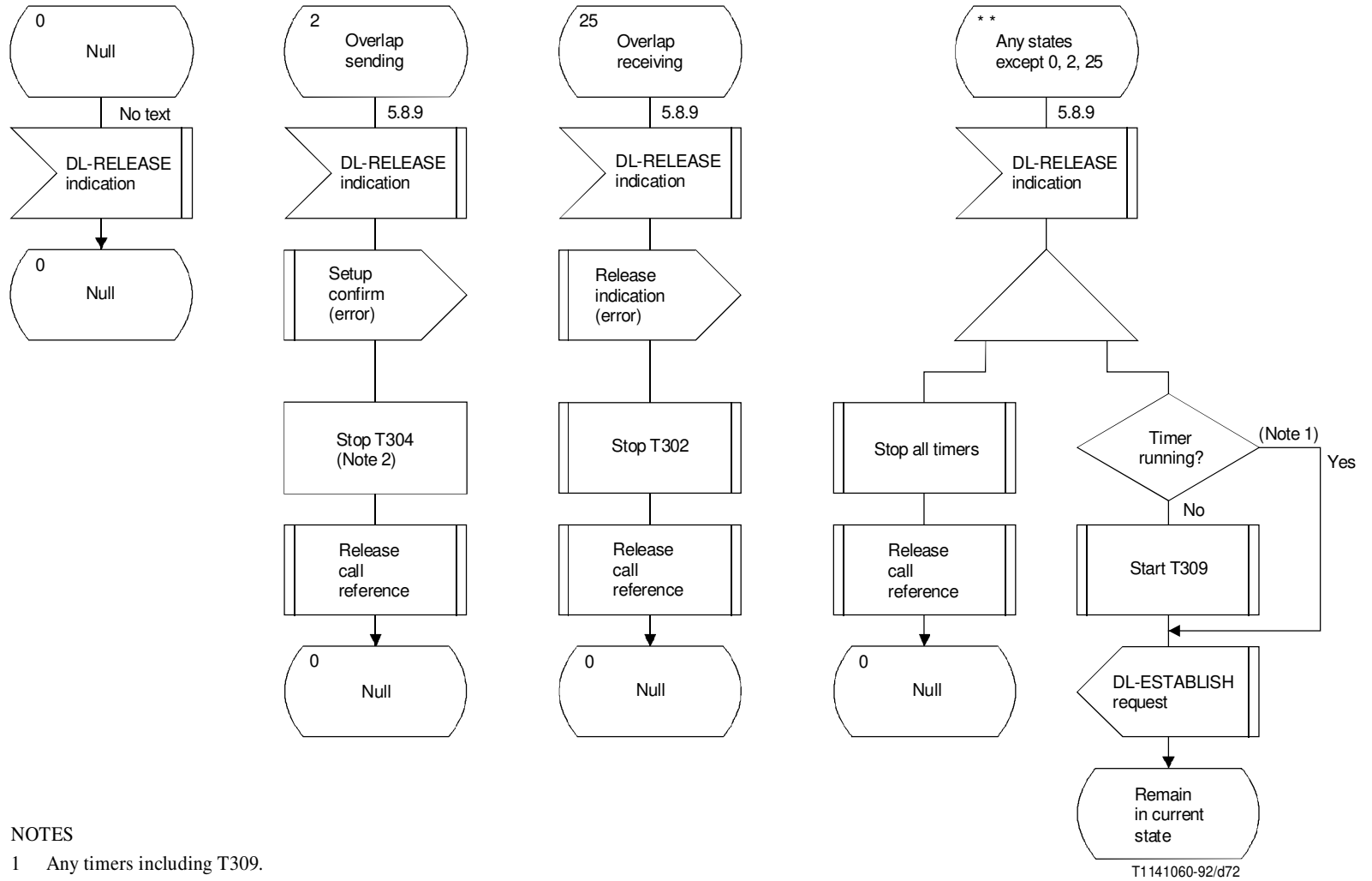
FIGURE A.6/Q.931 (Sheet 26 of 27) Detailed protocol control (network side) point-point
