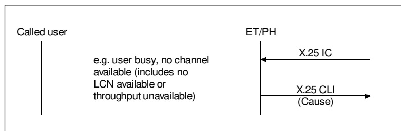
FIGURE II.8/Q.931
