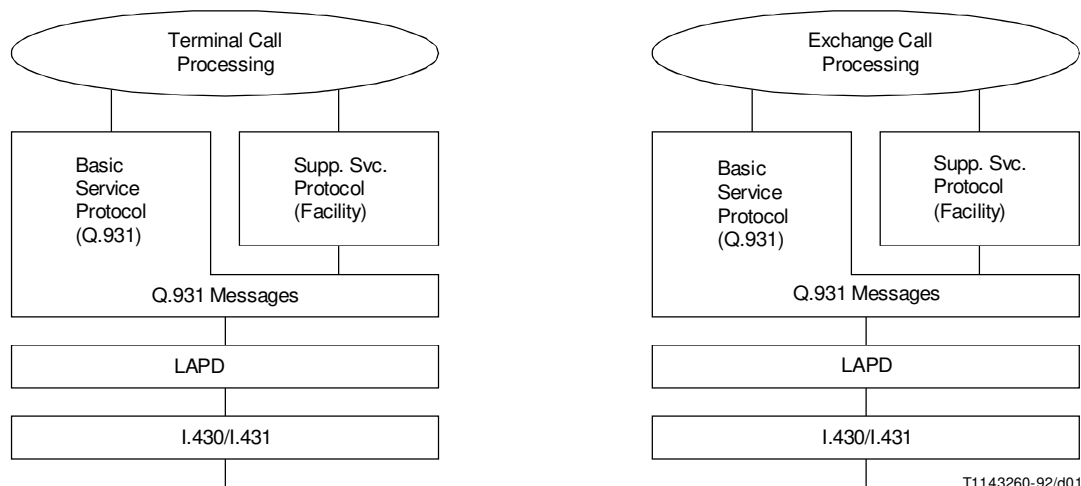
FIGURE 1/Q.930
