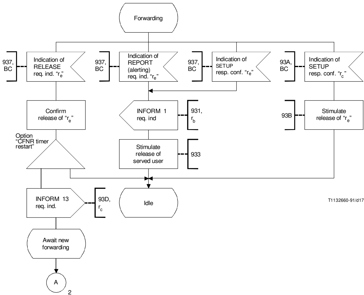
FIGURE 2-16/Q.82 (sheet 1 of 2)
