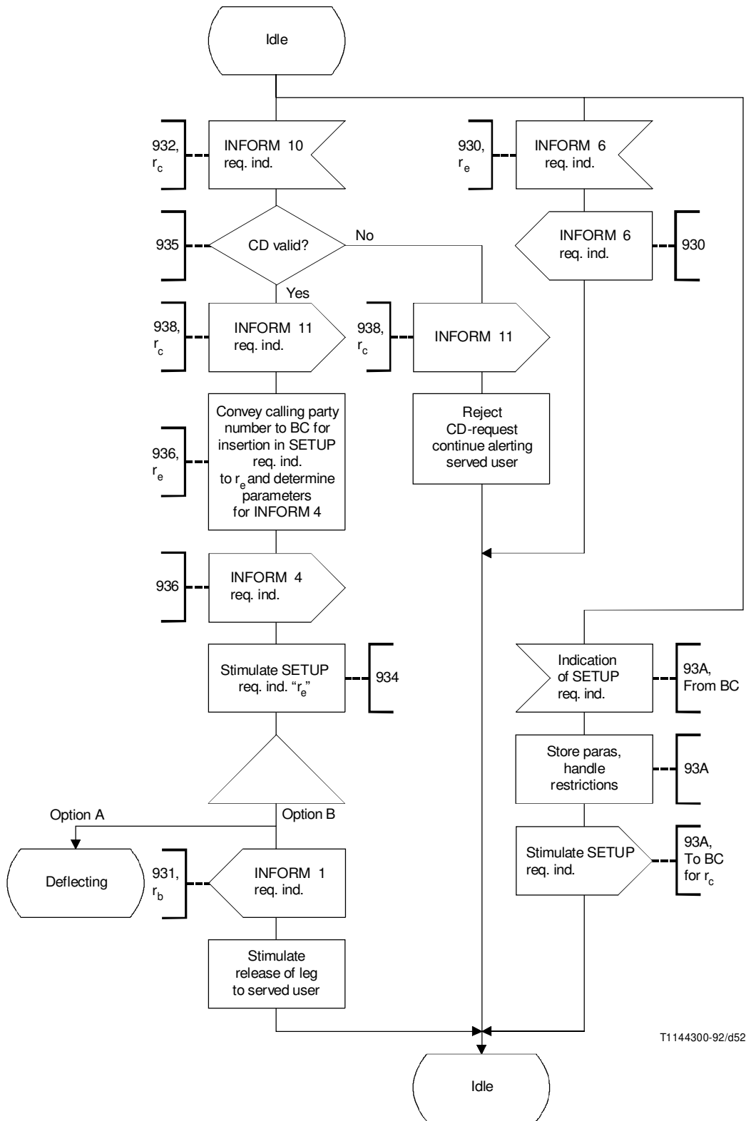
FIGURE 3-11/Q.82 (sheet 1 of 2)
