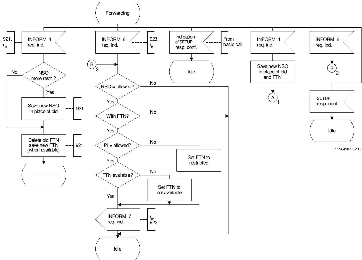
FIGURE 2-14/Q.82 (sheet 2 of 2) FE2. Call Diversion
