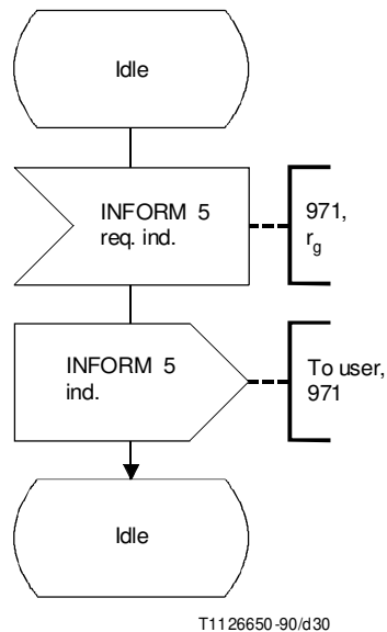
FIGURE 2-22/Q.82 FE7. Call Diversion
