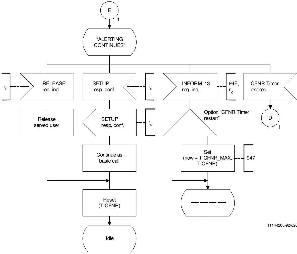
FIGURE 2-17/Q.82 (sheet 2 of 2)
