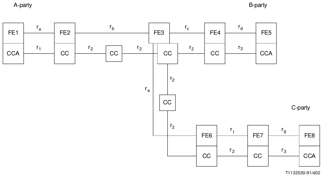
FIGURE 2-2/Q.82 Relationship with a basic service
