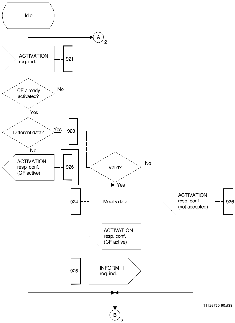
FIGURE B.2-6/Q.82 (sheet 1 of 2) SCE2 functions of supplementary service control
