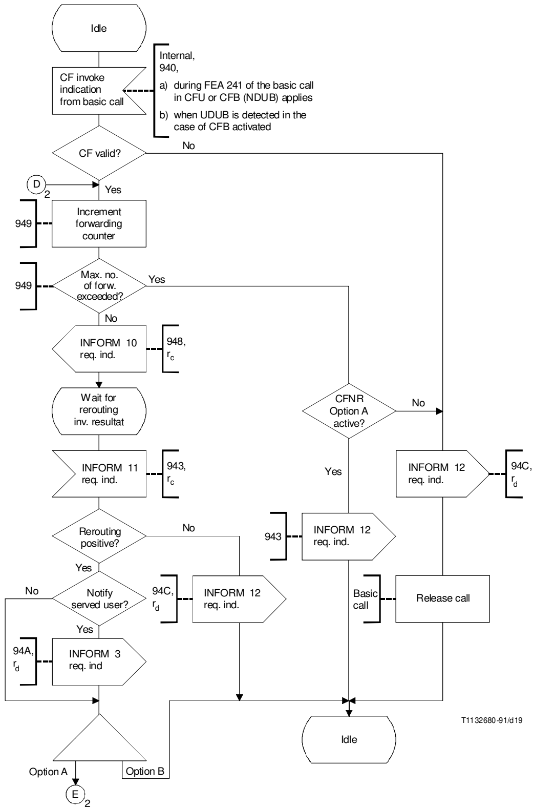
FIGURE 2-17/Q.82 (sheet 1 of 2)
