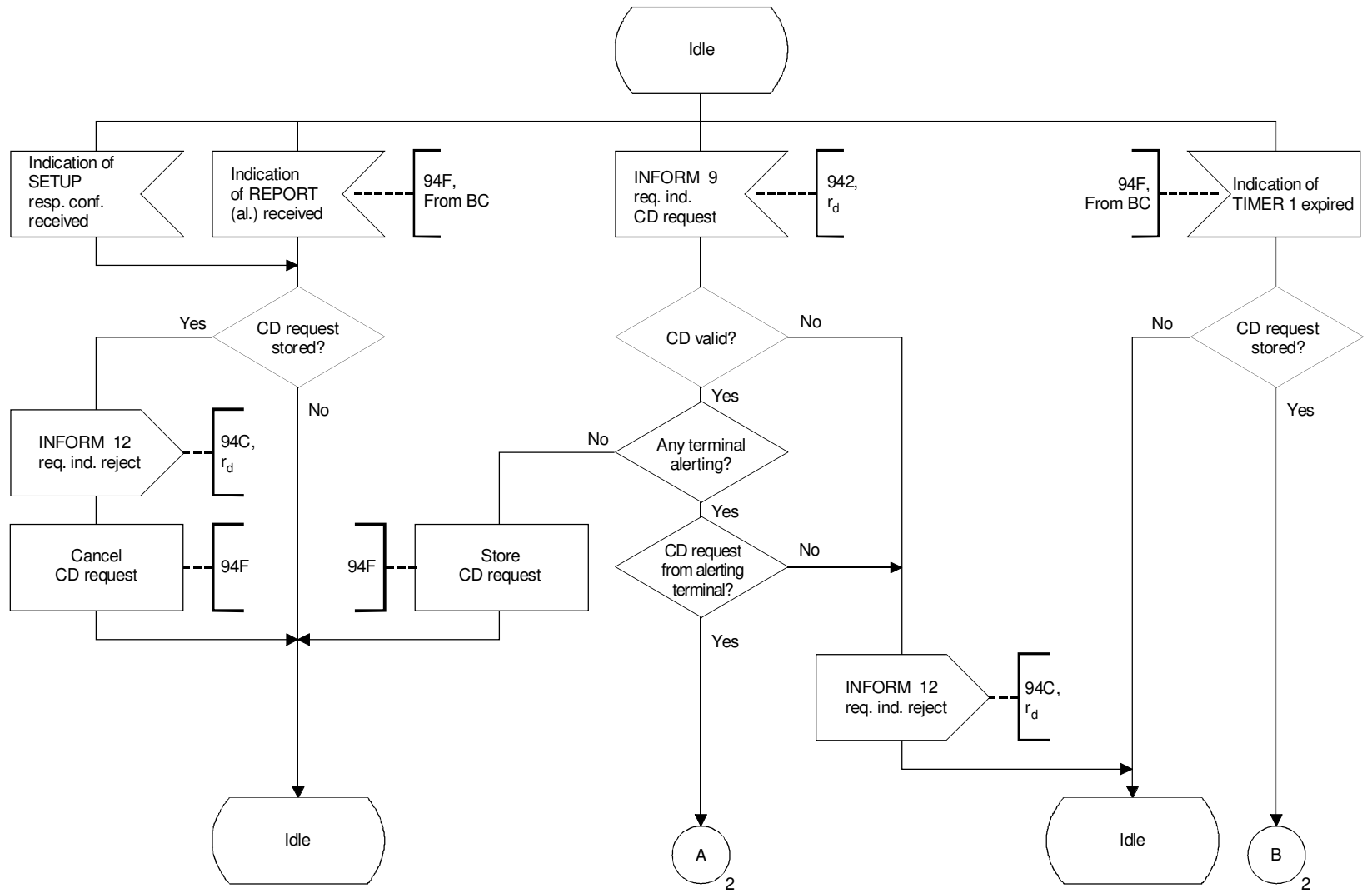
FIGURE 3-12/Q.82 (sheet 1 of 3) Functional entity FE4 call deflection
