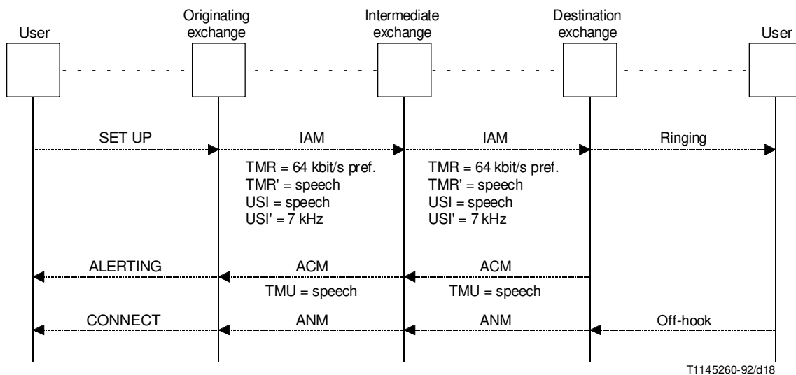
FIGURE D.4/Q.764 Fallback when called user is non-ISDN
