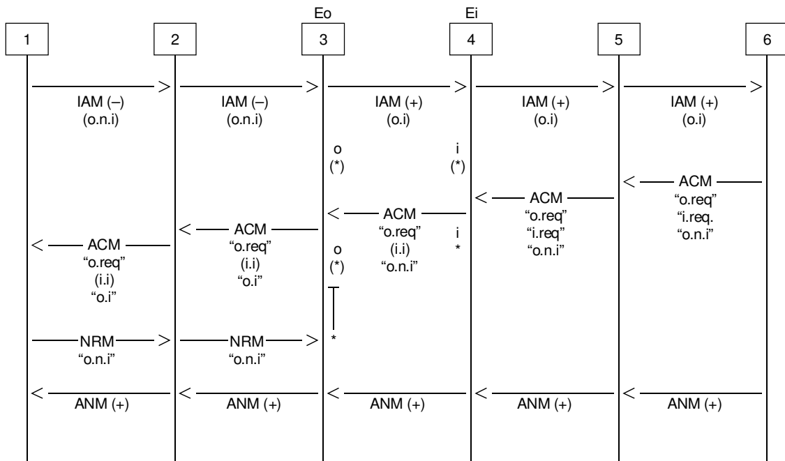
FIGURE C.3/Q.764
