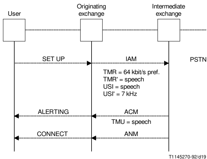
FIGURE D.5/Q.764 Fallback when interworking with PSTN
