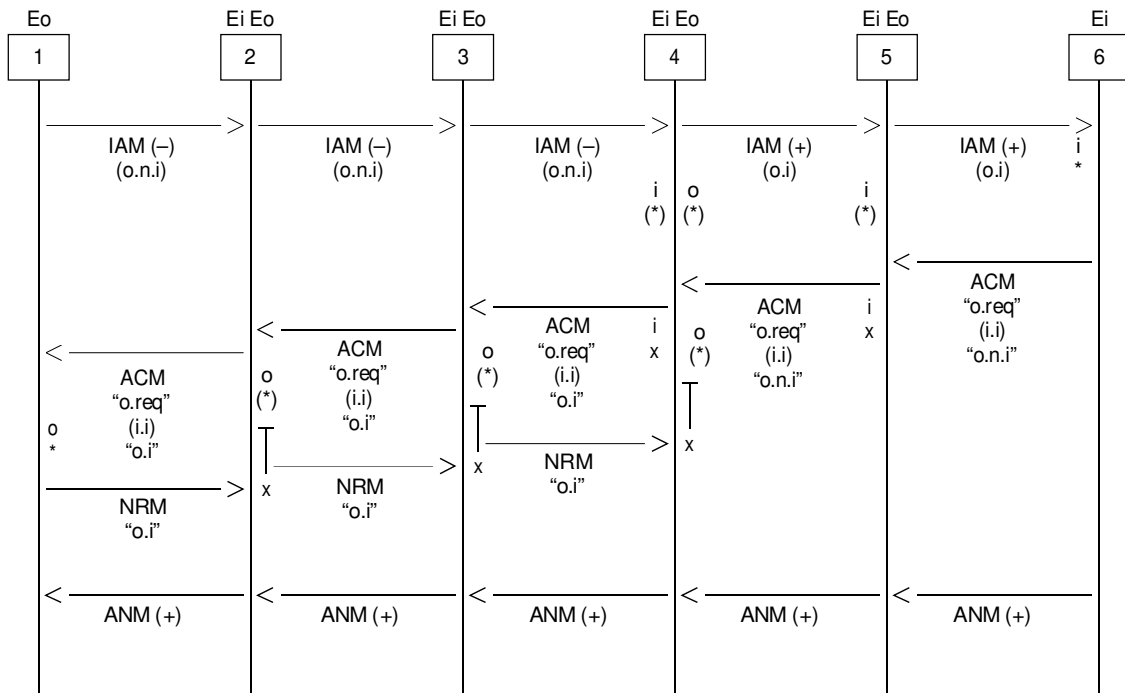
FIGURE C.1/Q.764
