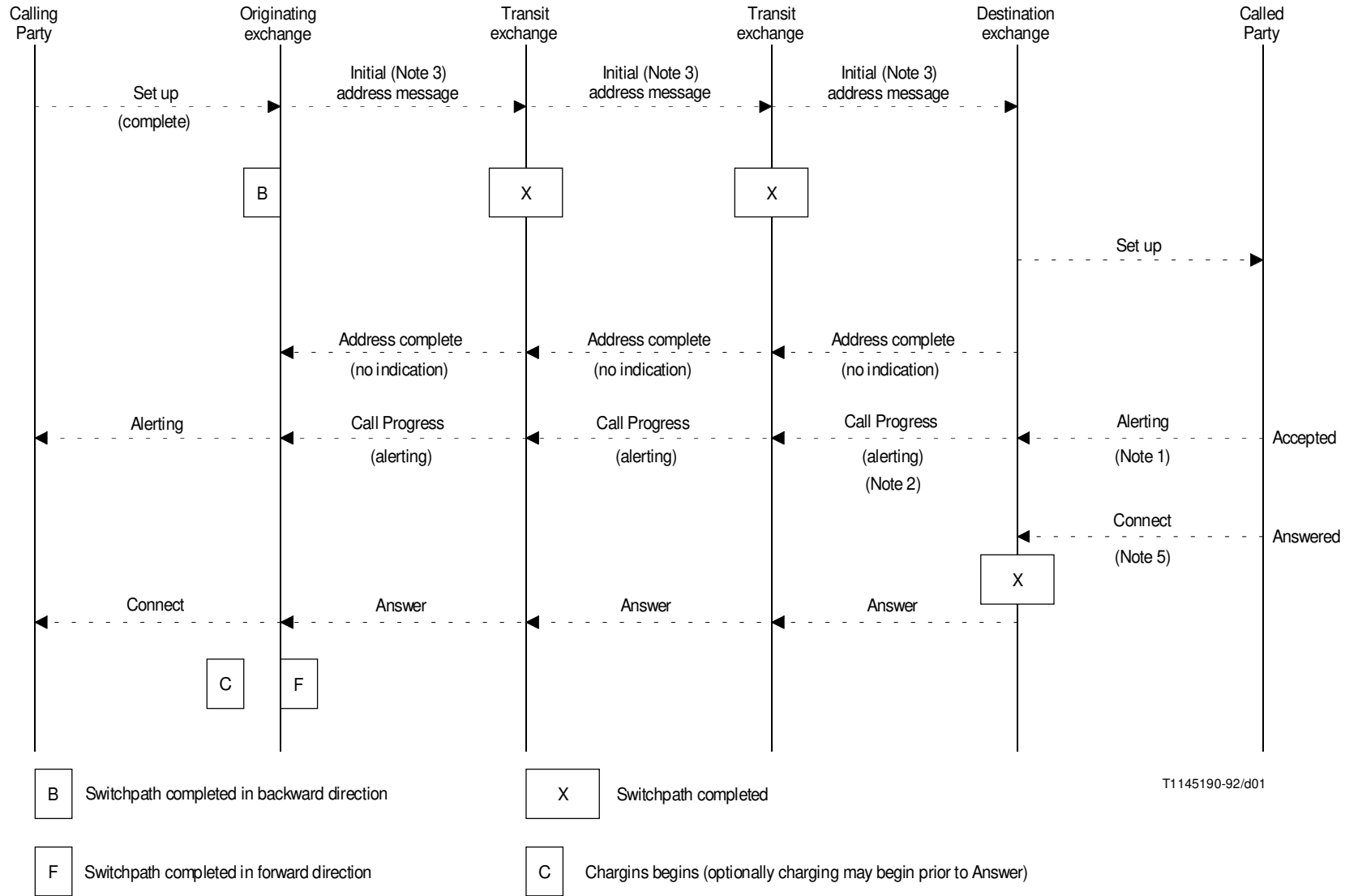
Annex B Figures on basic call control signalling procedures (This annex forms an integral part of this Recommendation)
