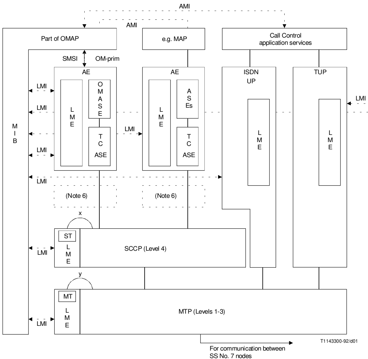
FIGURE 1/Q.755 SS No. 7 management and internal configuration of an SP
